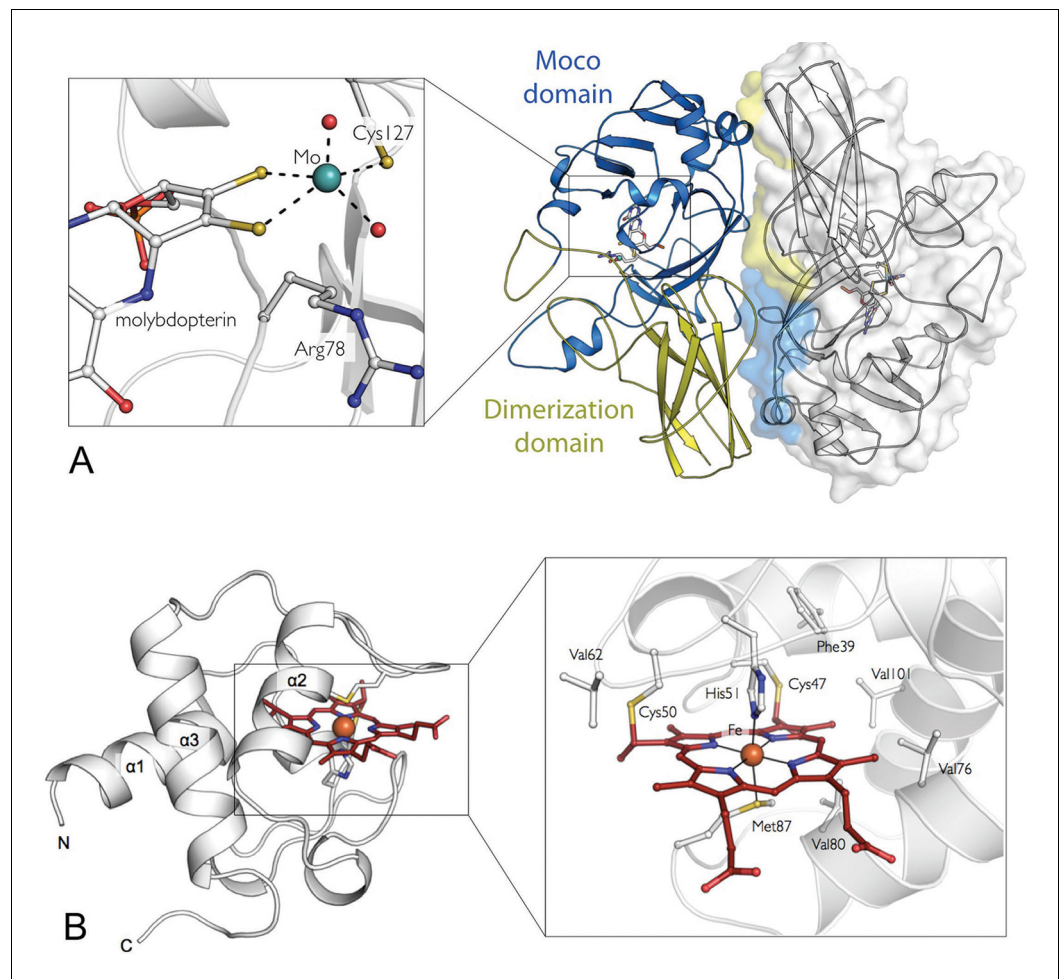
Figure 1. The crystal structures of the SorT and SorU proteins in isolation. (A) The structure of the SorT homodimer. Molecule A in blue/yellow; molecule B in gray (with transparent surface). For molecule A, the ‘SUOX-fold domain’ and ‘dimerization domain’ are represented in blue and yellow, respectively. The molybdopterin cofactor is shown as sticks within the SUOX-fold domain. The corresponding domains of the opposing protomer (shown in molecular surface representation), which constitute the dimer interface are colored to highlight the ‘head-to-tail’ dimer arrangement. INSET: a closer view of the molybdenum binding-site: the molybdenum atom (green sphere) is coordinated by two dithioline ligands from the molybdopterin (yellow spheres), residue Cys 127, an axial oxo ligand and an equatorial hydroxo or water ligand (red spheres). (B) The structure of SorU. The main three helices are labeled and the heme cofactor is shown in red. INSET: the heme binding site with the heme cofactor, coordinating residues, covalent links to Cys 50 and 57 and hydrophobic residues lining binding site: Phe 39, Val 62, Val 76, Val 80, Val 101 highlighted.
