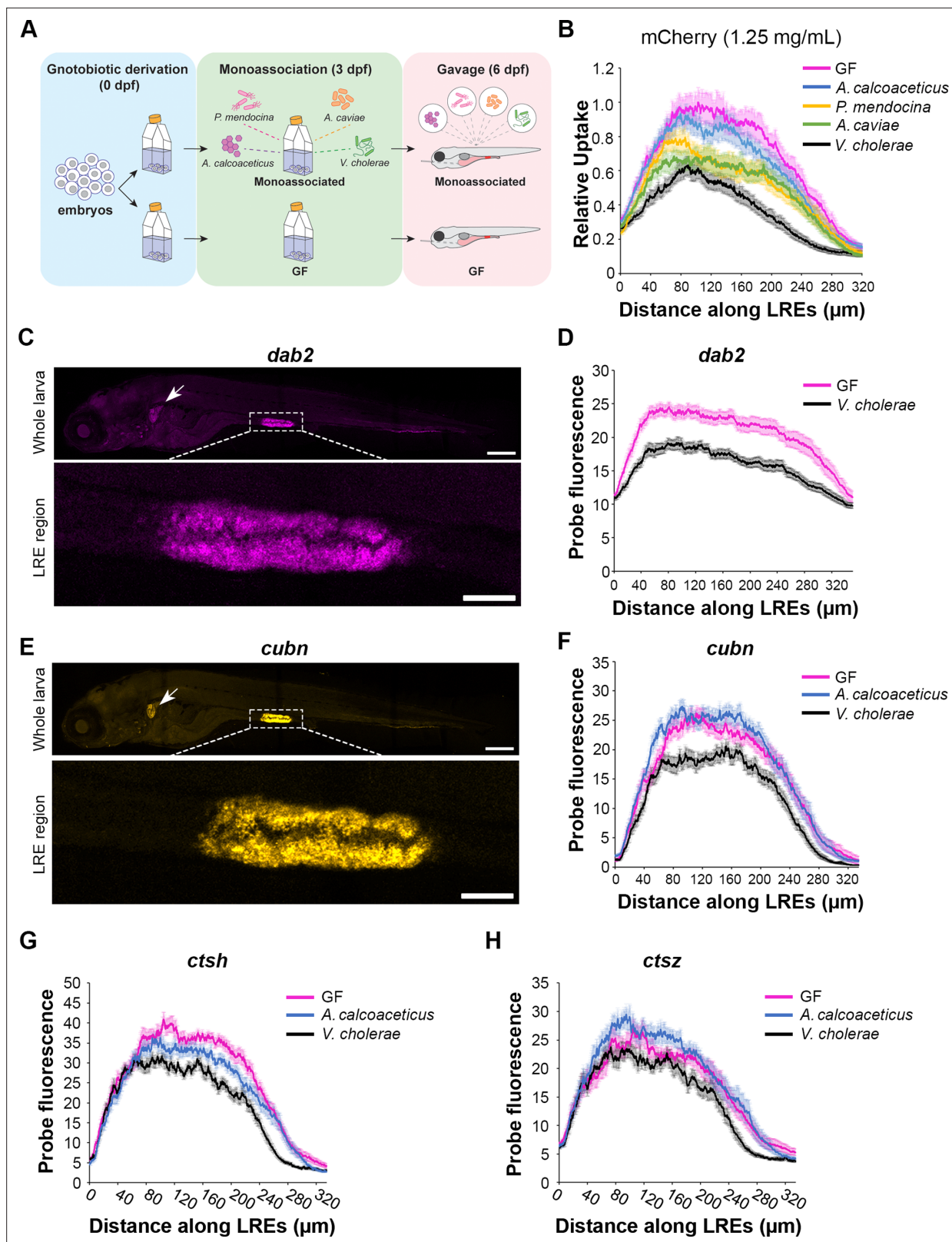
Figure 6. Lysosome-rich enterocyte (LRE) activity and expression of endocytic machinery are differentially affected by individual microbial strains. (A) Cartoon of monoassociation experimental design. Following gnotobiotic derivation, monoassociated larvae are colonized with a single strain of bacteria at 3 dpf and gavaged with mCherry to measure protein uptake at 6 dpf. (B) Plot shows relative uptake of mCherry in larvae that were germ-free (GF) or monoassociated with a single bacterial strain. mCherry uptake was reduced by A. calcoaceticus (two-way ANOVA, p=0.0268 , n=19-20 ), P. mendocina Figure 6 continued on next page
