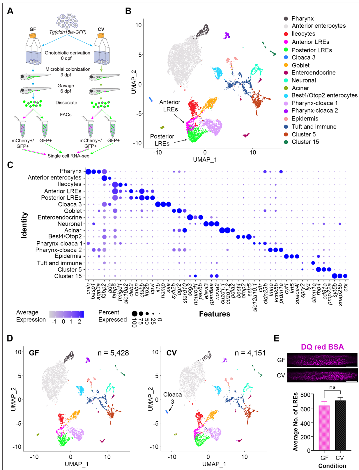
Figure 3. Single-cell clustering reveals anterior and posterior lysosome-rich enterocytes (LREs), microbially-responsive cloaca cells. (A) Cartoon depicting experimental design for transcriptomic profiling of intestinal cells in germ-free (GF) and conventional (CV) larvae. GF and CV larvae expressing Tg(cldn15la-GFP) to label all intestinal epithelial cells (IECs) were raised to 6 dpf in gnotobiotic conditions and then gavaged with mCherry (1.25 mg/mL). Cells from dissociated larvae were fluorescent-activated cell sorting (FACS) sorted to isolate GFP-positive/mCherry-negative from GFP-positive/mCherry-positive cells. (B) UMAP plot showing cell clusters. (C) Dot plot showing gene expression across cell identities. (D) UMAP plots for GF and CV conditions. (E) DQ red BSA staining and bar graph of Average No. of LREs.
