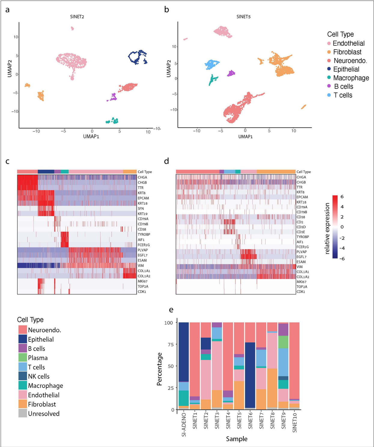
Figure 1. Cellular composition of small intestine neuroendocrine tumors (SiNETs) as determined by single-cell and single-nuclei sequencing. (A, B) UMAP plots showing the diversity of single cells from SiNET2 (A) and SiNET5 (B) , colored by their cluster assignment. (C, D) Cluster annotations (top bar) in SiNET2 (C) and SiNET5 (D) are supported by the expression of canonical cell type markers (rows). Also shown are three cell cycle markers (bottom rows). (E) Cell type frequencies in each of the 10 SiNETs that we profiled, along with one SiAdeno sample.
