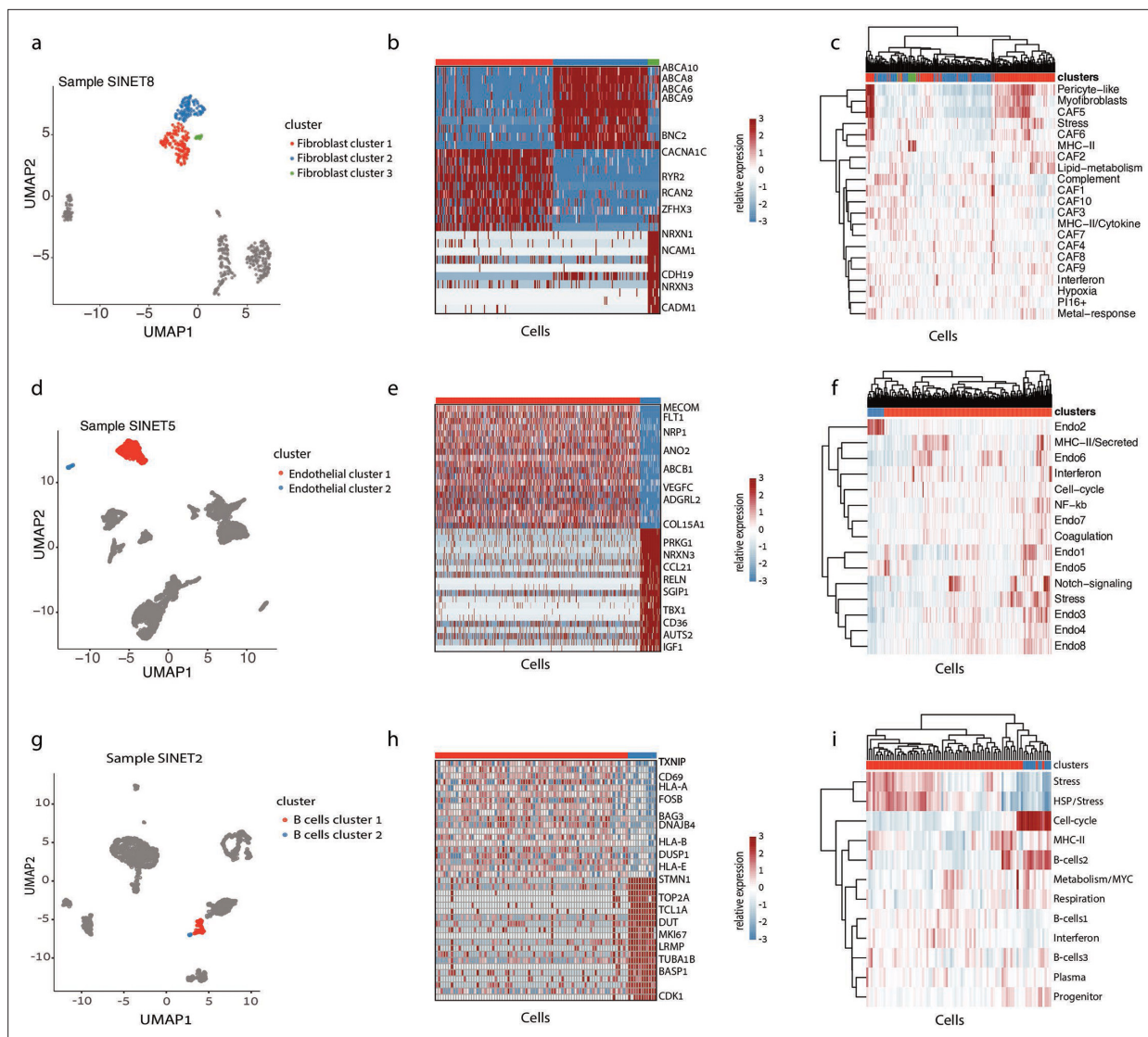
Figure 3. Heterogeneity in the small intestine neuroendocrine tumor (SiNET) microenvironment. For each of the three non-malignant cell types, the diversity of that cell type is shown in one exemplary tumor: fibroblast heterogeneity in SiNET8 is shown in (A–C), endothelial cell heterogeneity in SiNET5 is shown in (D–F), and B-cell heterogeneity in SiNET2 is shown in (G–I). For each cell type, three panels depict three types of analyses. The first panel (A, D, G) is a UMAP plot of the respective tumor, where only the respective cell type is colored, and distinct colors highlight the clusters of that cell type. The second panel (B, E, H) shows differential expression analysis between the first two clusters using heatmaps, with labeling of selected genes. The third panel (C, F, I) shows clustering of cells from that cell type (columns) based on their relative expression of previously defined (Gavish et al. , 2023) signatures of diversity in that cell type (rows); the top panel shows assignment of cells to clusters.
