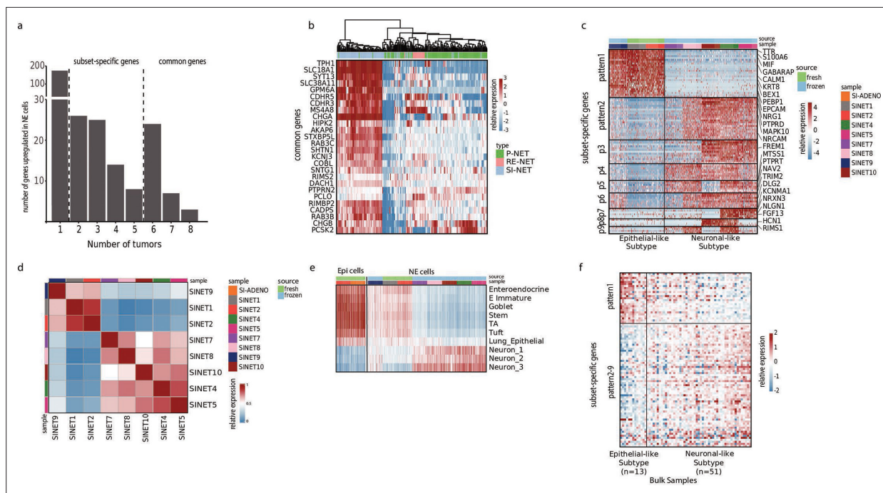
Figure 2. Small intestine neuroendocrine tumors (SiNETs) broadly classify into two major subtypes. (A) Bar plot showing the number of upregulated genes against a common threshold, number of genes (y-axis) vs number of tumors (x-axis). (B) Heat map showing a list of 25 representative genes that define SiNET signature of our single-nuclei RNA sequencing (scRNA-seq) cohort used to cluster neuroendocrine tumor (NET) samples from a bulk-seq dataset (Alvarez et al., 2018). Type of NET is color-coded on the top panel, with P-NET and RE-NET referring to pancreatic and rectal NETs. (C) Heatmap representing clustering of SiNET samples in our cohort based on genes that were differentially expressed and shared between 2–5 samples, showing two major variable gene programs. (D) Correlation heat map between the NET samples. (E) Heatmap showing average expression of epithelial and neuronal gene sets (rows) in the neuroendocrine and epithelial cells from our SiNET samples (columns). Epithelial gene sets include signatures of multiple cell types from the small intestine (Haber et al., 2017), and neuronal gene sets include three clusters of neurons (Mahalingam et al., 2020). (F) Heatmap of the SiNET-dominated cluster from the bulk dataset (Alvarez et al., 2018) was subjected to differential expression analysis using the same set of genes as (C).
