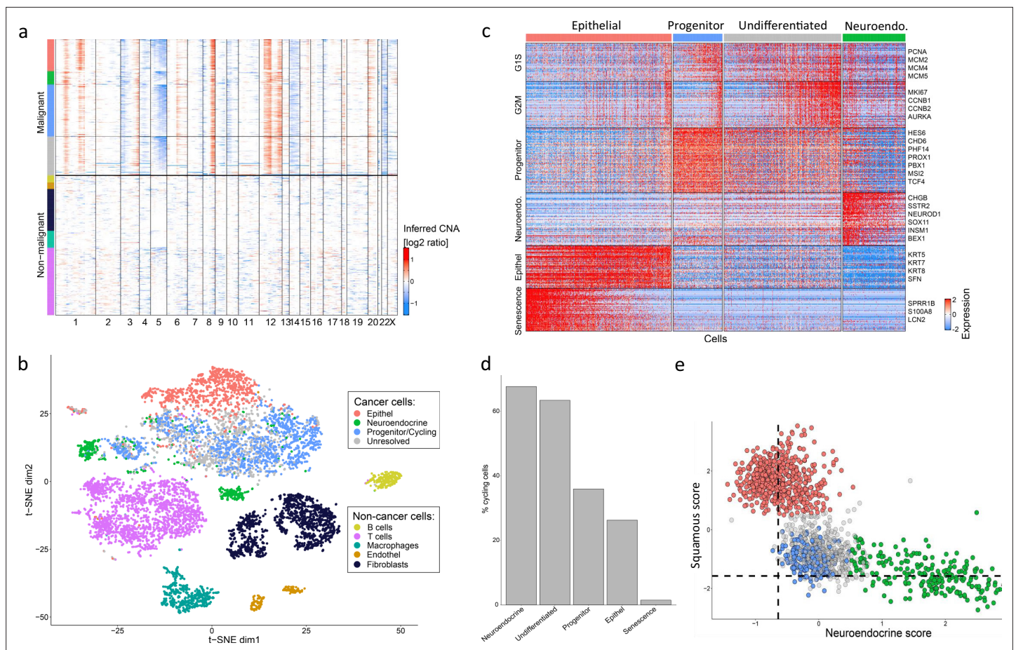
Figure 5. A putative progenitor population in mixed Large Cell Neuroendocrine Carcinoma (LCNEC). (A) Copy number variation (CNV) profiles inferred from single-nuclei RNA sequencing (scRNA-seq) data for all cells from the LCNEC sample. Malignant and non-malignant cells are annotated based on their CNV profiles, using the same color codes as in the next panels. (B) tSNE plot showing the diversity of single cells from the mixed lung tumor, colored by their clustering. (C) Heatmap shows relative expression of differentially expressed genes (rows), separated by horizontal lines into programs that distinguish between the four populations of cells detected in the LCNEC sample. Also included are two cell cycle programs (G1/S and G2/M). Columns correspond to malignant cells, separated into the four populations by vertical lines and as indicated by color at the top. Selected genes are labeled for each program. (D) Bars show the percentage of cycling cells in each malignant cluster. (E) Malignant cells scored against an epithelial vs. neuroendocrine program (gene set), colored by their assignment into four populations.
