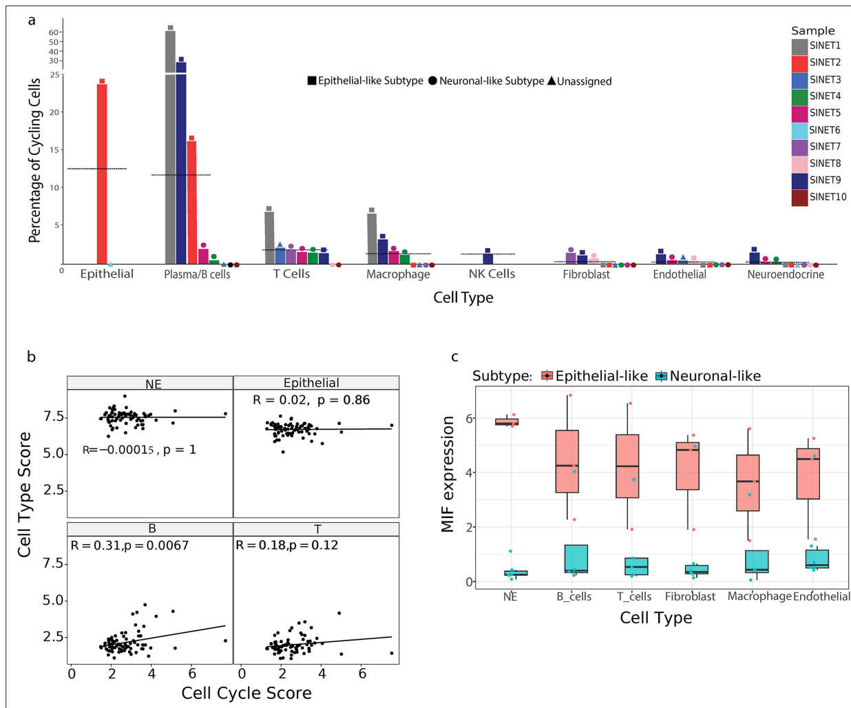
Figure 4. Cell cycle analysis reveals proliferating B cells in small intestine neuroendocrine tumors (SiNETs). (A) Bars show the percentage of cycling cells (y-axis) per cell type and per tumor (x-axis). Tumors are color-coded, the two subtypes, epithelial-like and neuronal-like, are differentiated by distinct shapes, represented as square and circle, respectively. Information regarding the presence of cell types with zero percentage of cycling cells is provided along the x-axis. Horizontal lines indicate average percentages of cycling cells per cell type. (B) Correlation between cell type and cell-cycle program as computed from an SiNET bulk RNA-seq dataset ( Alvarez et al., 2018 ). Score for each cell type is represented at the top of individual panels. (C) Boxplot depicting the expression of migration inhibitory factor (MIF) in each SiNET cell type, for each of the two SiNET subtypes.
