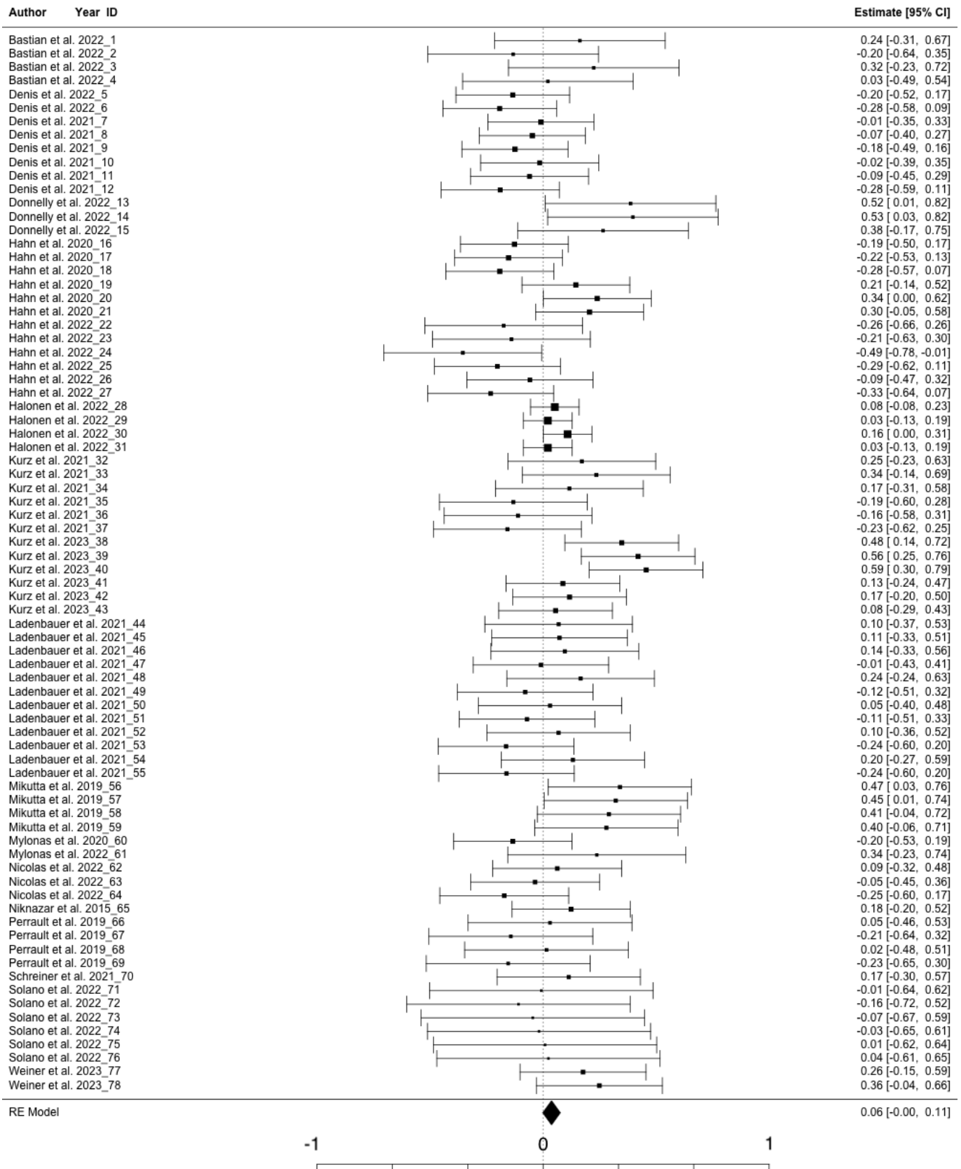
Figure 2: SP amplitude frequentist forest plot
