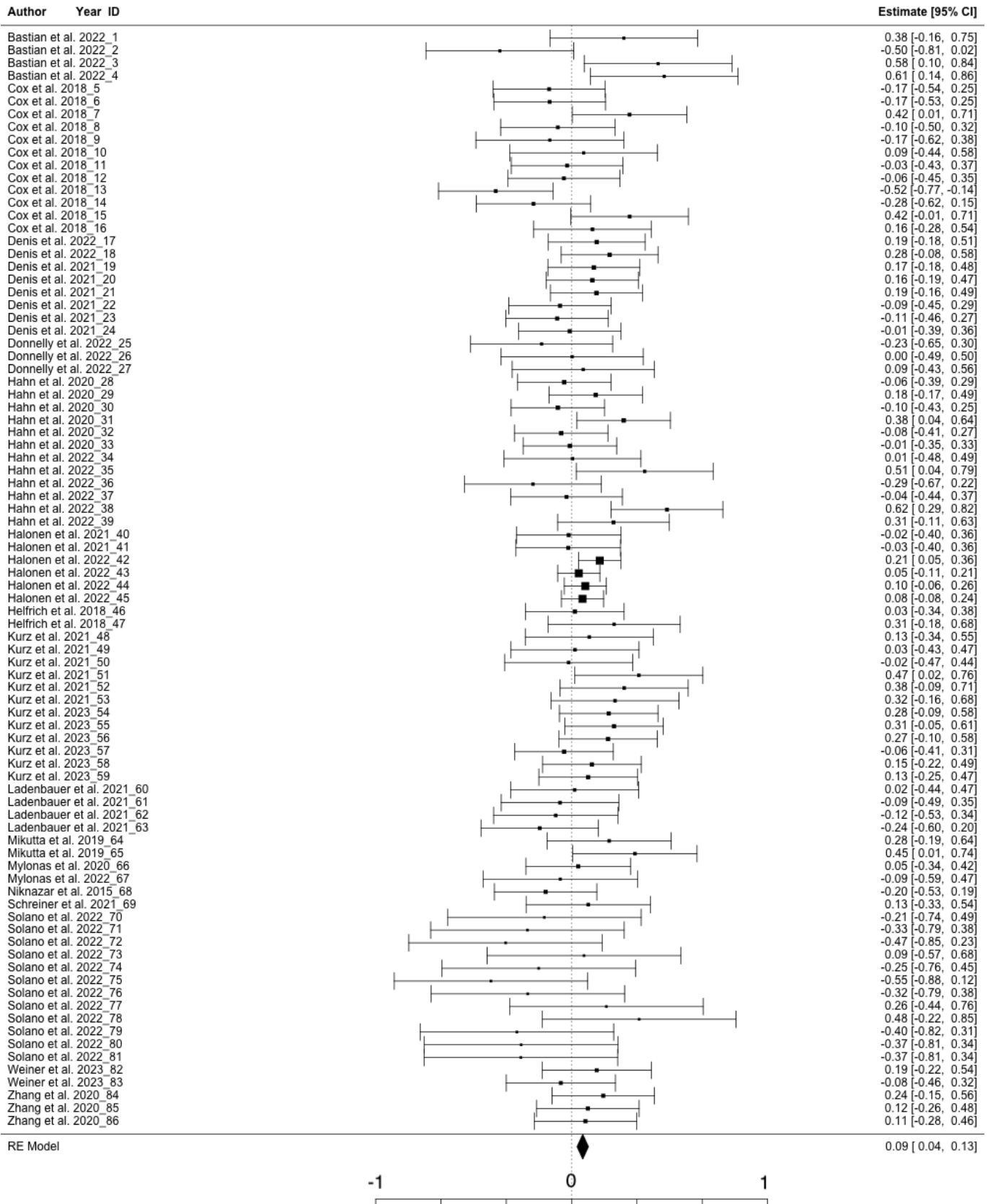
Figure 3: Coupling strength frequentist forest plot
