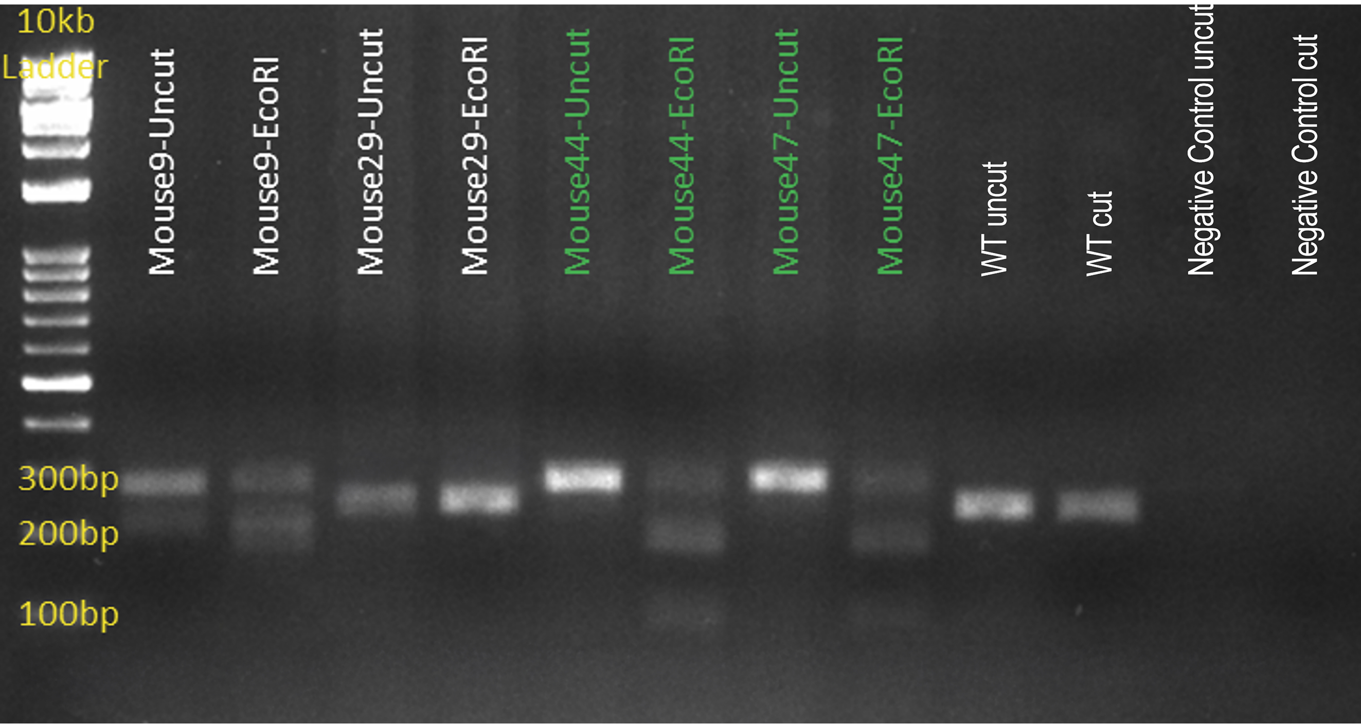
Tbx5 locus (3' arm + Lox2272 insert - cut with SphI )
