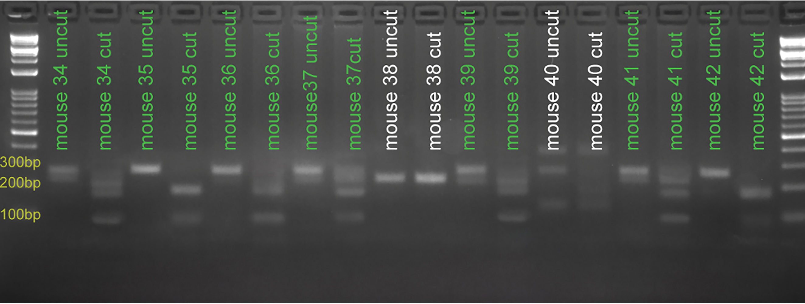
Tbx5 locus (5' arm + Lox2272 insert - cut with EcoRI )
