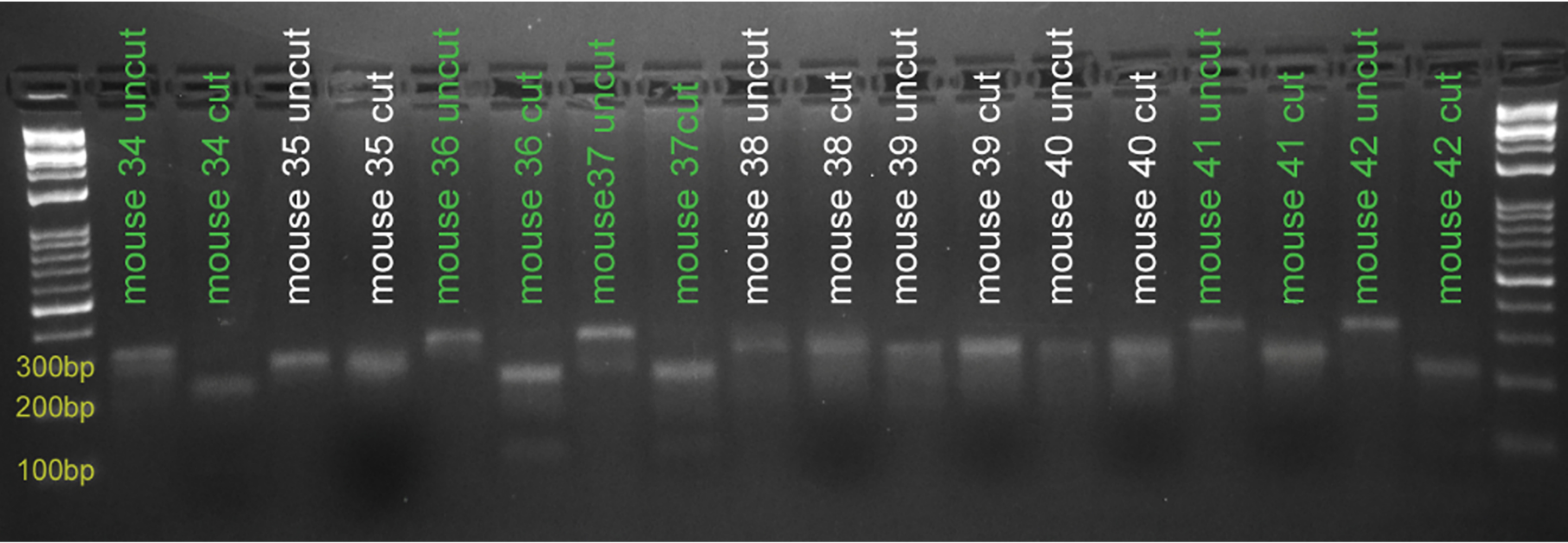
Tbx5 locus (3' arm + Lox2272 insert - cut with SphI )
