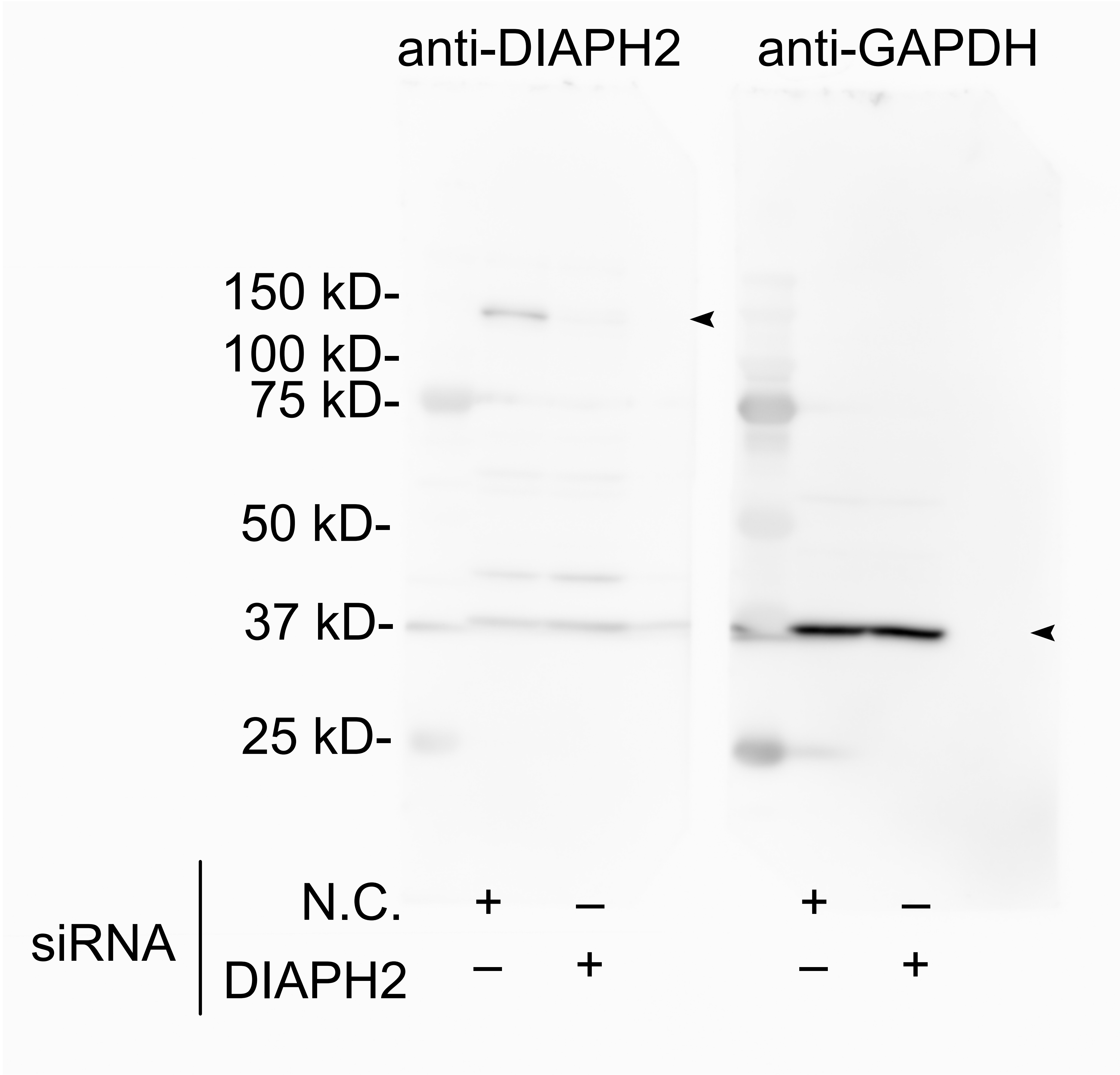
Figure 2 – figure supplement 2, Source Data 1. Original membranes corresponding to Figure2 – figure supplement 2B and C. siRNA treatments are indicated below each lane. Arrowheads mark the bands of interest. these bands are shown with contrast adjustment in Figure 2—figure supplement 2B–C.
