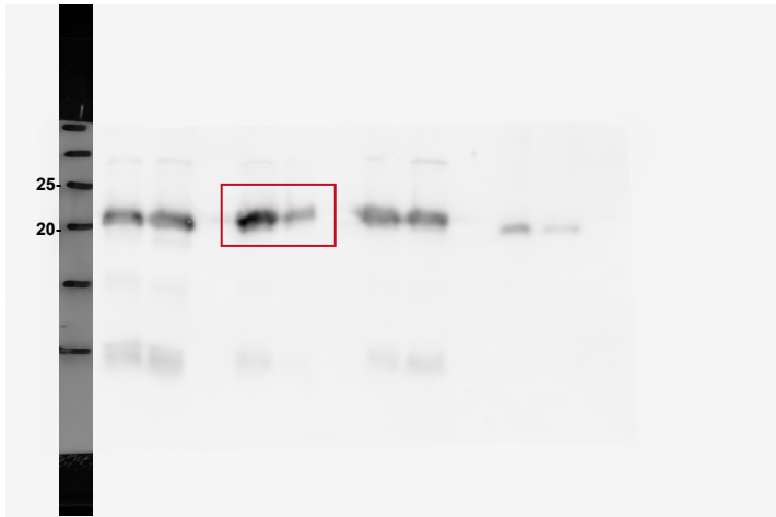
anti-claudin-1
