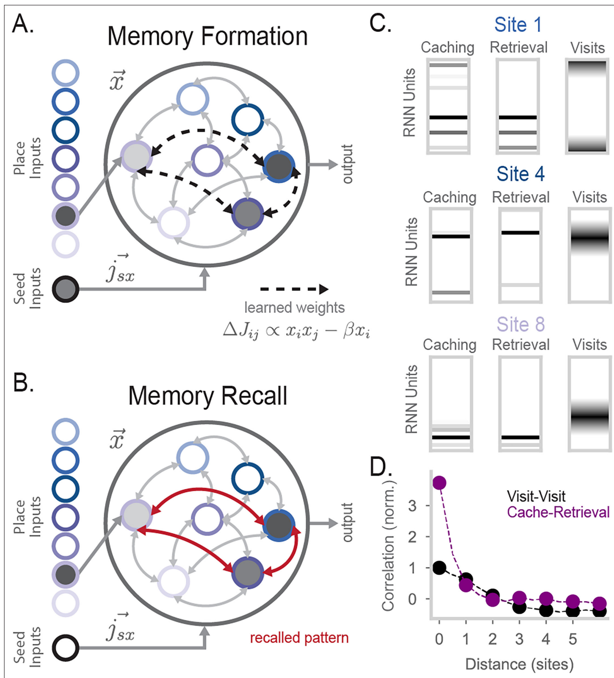
Figure 3. Barcode activity binds content to store memories in the RNN. (A) Diagram of RNN activity during memory formation. Along with place inputs, a scalar seed input s is provided to the model. s connects to RNN units via 5000-dimensional weight vector \vec{j}_{sx} \sim \mathcal{N}(0, 1) . During memory formation (i.e. when an animal caches a seed), place inputs representing the animal's current location and a seed input are provided to the RNN. After recurrent dynamics are run for some time ( t = 100 ), the network undergoes Hebbian learning. (B) An example of memory recall in the network. The animal is at the same location as in (A) . The place input encoding that location is provided to the model and results in the RNN recalling the stored attractor pattern seen in (A) . (C) Examples of RNN population activity during caching (left), retrieval (center), and visits (right) at three sites. During visits, the RNN has r = 0 , while during caches and retrievals r = 1 . For visualization purposes, 50 units are randomly sampled and displayed in the 'Caching' and the 'Retrieval' plot. (D) Correlation of Poisson-generated spikes simulated from RNN rate vectors at two sites, plotted as a function of the distance between the two sites. In black is the correlation in activity between two visits. In purple is the correlation between caching and retrieval activity. Experiments were simulated with 20 simulations where 5 sites were randomly chosen for caching and retrieval. 99% confidence intervals are calculated over the simulations and plotted over the markers. Compare to Figure 1E and F .
