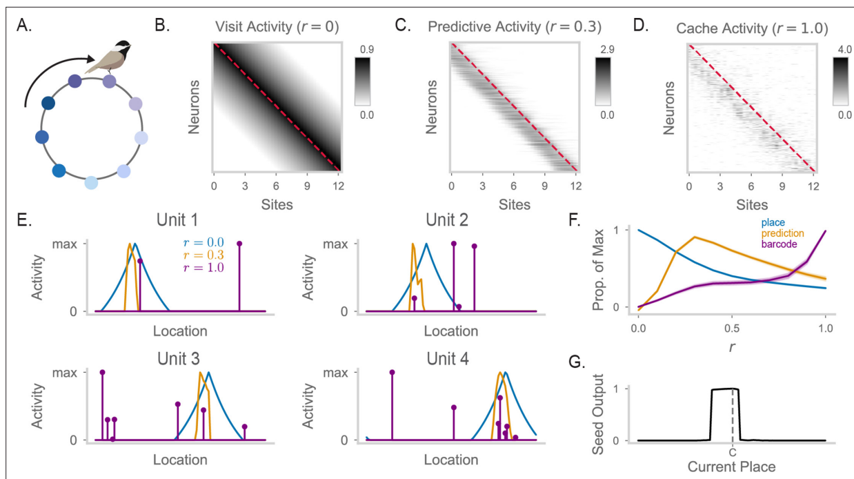
Figure 6. Predictive coding and barcode generation are performed by the same RNN in different dynamical regimes. (A) Cartoon of a chickadee in a circular track, running in a consistently clockwise direction. (B) Heatmap of RNN firing fields when r = 0 , where each row corresponds to the tuning curve of one neuron across all locations. Red dashed line indicates the diagonal. (C) As in (B), but for r = 0.3 . Here, clockwise movement corresponds to movement from site i to site i + 1 . Thus, predictive activity appears as a shift in RNN activity below the matrix diagonal. (D) As in (B), but for r = 1.0 . Barcodes appear as random, off-diagonal structure in the activity matrix. (E) The firing fields of four example units across different recurrent strengths. That is, each unit's row in (B) is in blue, its row in (C) is in orange, and its row in (D) is in purple. Each curve is max-normalized. (F) Average projection strength of RNN activity onto the place code, predictive code, and barcode vectors. The place code vector is defined as activity with r = 0 . The predictive code vector is defined as the place field of the unit at the next clockwise site, minus the projection onto the place code. The barcode vector is defined as activity with r = 1.0 , minus the projection onto the place code. Lines show the mean over the 100 units of the mode, with shading displaying 99% confidence interval. Each line is max-normalized. (G) Seed output of the model with predictive weights, given the animal's location on the circular track. Here, there is only one cache, made at the halfway location of the circular track (labeled "C").
