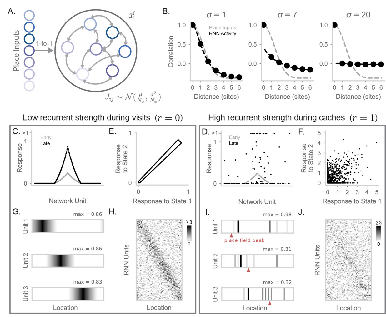
Figure 2. A recurrent neural network generates barcode activity through recurrent dynamics. (A) Diagram of a RNN; the activity of the network units is denoted as \vec{x} . Place information arrives from an input layer with activities \vec{p} . Recurrent weights are initialized randomly, that is, J_{ij} \sim \mathcal{N}(\frac{\mu}{N_x}, \frac{\sigma^2}{N_x}) for the synapse connecting neuron j to neuron i , where N_x is the number of RNN neurons. (B) Correlation of activity vectors across different locations, when RNN weights are initialized with \sigma = 1 (left), \sigma = 7 (center), and \sigma = 20 (right). We show correlation of place inputs (gray) and correlation of the RNN's rate vector at t = 100 (black). X-axis is in units of site distance (see Methods for definition). (C) Response of RNN units when simulating a visit to a location halfway around the circular track (with r = 0 ; equation 3). In gray is the activity of the RNN at t = 1 . In black is the activity at t = 100 RNN units that are uniformly subsampled and sorted by the tuning of their inputs for plotting purposes. (D) As in (C) , but for r = 1 . RNN activity is more sparsely distributed, including high activity in neurons without place tuning for the current location. For visualization purposes, 50 RNN units with nonzero activity and 50 RNN units with 0 activity are sampled at this time point ( t = 100 ) for display, and responses greater than 1 are clipped to > 1 . (E) RNN activity in response to state 1 compared to state 2, when r = 0 . Each point corresponds to a single RNN unit. (F) As in (E) , but for r = 1 . RNN activity for these neighboring states is substantially decorrelated by recurrence. (G) Firing fields of three example units on the circular track displaying place-cell activity. Maximum value of each field is labeled and the colormap is max-normalized. (H) Simulated spike counts of a RNN population during visits to each location on the circular track. Spikes are generated by simulating Poisson-distributed counts from underlying unit rates. Place tuning results in a strong diagonal structure when units are sorted by their input's preferred location. The maximum limit of the colormap is set to the 99th percentile value of spike counts ( \geq 3 spikes). (I) Same neurons as (G) , but for r = 1 with units now showing barcode activity. The location of the r = 0 place field peak of each unit (i.e. its corresponding peak in (G) ) is marked by a red triangle. (J) As in (H) , but for r = 1 . The independence of barcode activity for neighboring sites results in a matrix with reduced diagonal structure.
