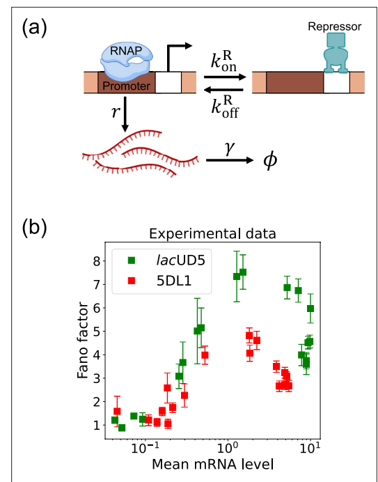
Figure 3. Two-state gene regulation architecture. (a) Schematic of gene regulatory circuit for transcriptional repression. RNA polymerase (RNAP) binds to the promoter region to initiate transcription at a rate r , leading to the synthesis of mRNA molecules (red wavy lines). mRNA is degraded at a rate \gamma . A repressor protein can bind to the operator site, with association and dissociation rates k_{on}^R and k_{off}^R , respectively. (b) Experimental data from Phillips et al., 2019, showing the relationship between the mean mRNA level and the Fano factor for two different promoter constructs: lacUD5 (green squares) and 5DL1 (red squares).
