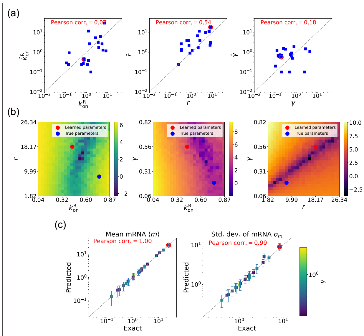
Figure 6. Gradient-based learning via differentiable Gillespie algorithm (DGA) is applied to the synthetic data for the gene expression model in Figure 3a . Parameters k_{off}^R are fixed at 1, with 1/a = 200 and 1/b = 20 for a simulation time of 10. (a) Scatter plot of true versus inferred parameters ( k_{on}^R , r , and \gamma ). Error bars are 95% confidence intervals (CIs). Panel (b) plots the logarithm of the loss function near a learned parameter set (shown in red circles in (a)), showing insensitivity regions. Panel (c) compares true and predicted mRNA mean and standard deviation with 95% CIs.
