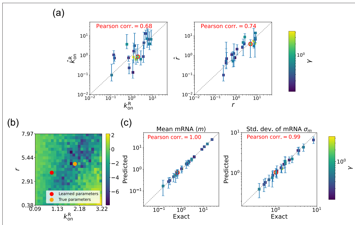
Figure 5. Gradient-based learning via differentiable Gillespie algorithm (DGA) is applied to the synthetic data for the gene expression model in Figure 3a . Parameters k_{off}^R are fixed at 1, with 1/a = 200 and 1/b = 20 for a simulation time of 10. (a) Scatter plot of true versus inferred parameters ( k_{on}^R and \hat{r} ) with \gamma constant. Error bars are 95% confidence intervals (CIs). Panel (b) plots the logarithm of the loss function near a learned parameter set (shown in red circles in (a)), showing insensitivity regions. Panel (c) compares true and predicted mRNA mean and standard deviation with 95% CIs.
