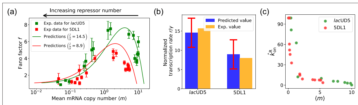
Figure 7. Fitting of experimental data from Jones et al., 2014 using the differentiable Gillespie algorithm (DGA). (a) Comparison between theoretical predictions from the DGA (solid curves) and experimental values of mean and the Fano factor for the steady-state mRNA levels are represented by square markers, along with the error bars, for two different promoters, lacUD5 and 5DL1 . Solid curves are generated by using DGA to estimate \hat{r} , \hat{\gamma} , and \{\hat{k}_{\text{on}}^R\} and using this as input to exact analytical formulas. (b) Comparison between the inferred values of \hat{r}/\hat{\gamma} using DGA with experimentally measured values of this parameter from Jones et al., 2014 . (c) Inferred \hat{k}_{\text{on}}^R values as a function of the mean mRNA level.
