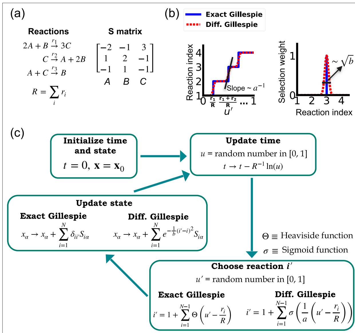
Figure 1. Comparison between the exact Gillespie algorithm and the differentiable Gillespie algorithm (DGA) for simulating chemical kinetics. (a) Example of kinetics with N = 3 reactions with rates r_i (i = 1, 2, 3) . (b) Illustration of the DGA's approximations: replacing the non-differentiable Heaviside and Kronecker delta functions with smooth sigmoid and Gaussian functions, respectively. (c) Flow chart comparing exact and differentiable Gillespie simulations.
