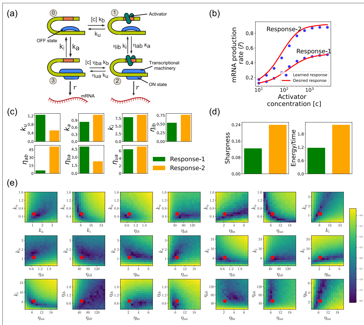
Figure 8. Design of the four-state promoter architecture using the differentiable Gillespie algorithm (DGA). (a) Schematic of four-state promoter model. (b) Target input–output relationships (solid curves) and learned input–output relationships (blue dots) between activator concentration [c] and average mRNA production rate. (c) Parameters learned by DGA for the two responses in (b) . (d) The sharpness of the response \frac{d\langle r \rangle}{d[c]} and the energy dissipated per unit time for two responses in (b) . (e) Logarithm of the loss function for the learned parameter set for Response-2, revealing directions (or curves) of insensitivity in the model's parameter space. The red circles are the learned parameter values.
