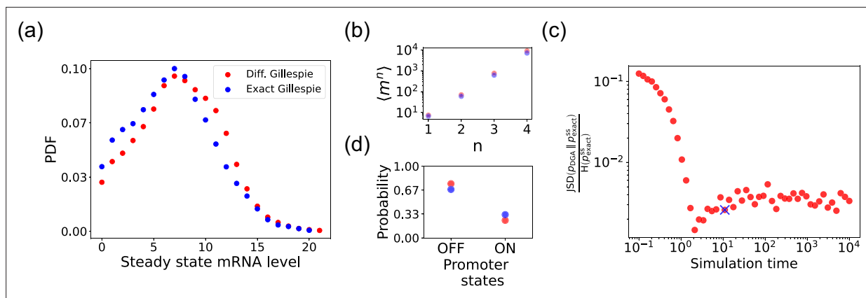
Figure 4. Accuracy of the differentiable Gillespie algorithm (DGA) in simulating the two-state promoter architecture in Figure 3a . Comparison between the DGA and exact simulations for (a) steady-state mRNA distribution, (b) moments of the steady-state mRNA distribution, and (d) the probability for the promoter to be in the 'ON' or 'OFF' state. (c) Ratio of the Jensen–Shannon divergence JSD(p_{DGA} || p_{exact}^{ss}) between the differentiable Gillespie probability distribution function (PDF) p_{DGA} and the exact steady-state PDF p_{exact}^{ss} , and the Shannon entropy H(p_{exact}^{ss}) of the exact steady-state PDF. In all of the plots, 2000 trajectories are used. The simulation time used in panels (a), (b), and (d) is marked by blue 'x'. Parameter values: k_{on}^R = 0.5 , k_{off}^R = 1.0 , r = 10 , \gamma = 1 , 1/a = 200 , and 1/b = 20 .
