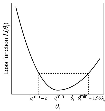
Appendix 3—figure 1. Error bars estimation for asymmetric loss function.
