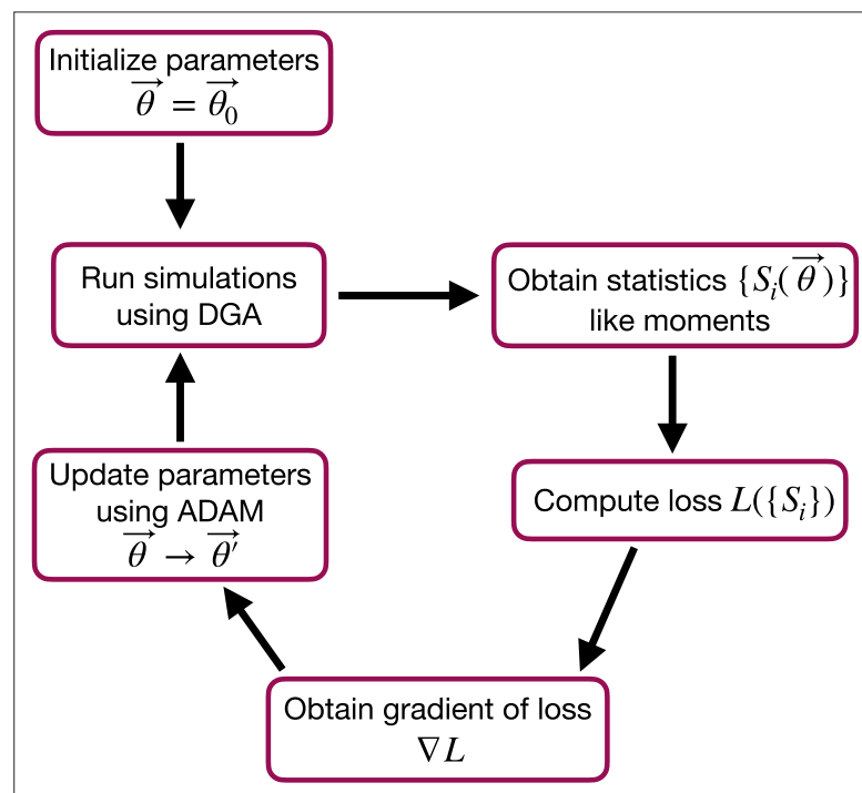
Figure 2. Flow chart of the parameter optimization process using the differentiable Gillespie algorithm (DGA). The process begins by initializing the parameters \vec{\theta} = \vec{\theta}_0 . Simulations are then run using the DGA to obtain statistics \{S_i(\vec{\theta})\} like moments. These statistics are used to compute the loss L(\{S_i\}) , and the gradient of the loss \nabla L is obtained. Finally, parameters are updated using the ADAM optimizer, and the process iterates to minimize the loss.
