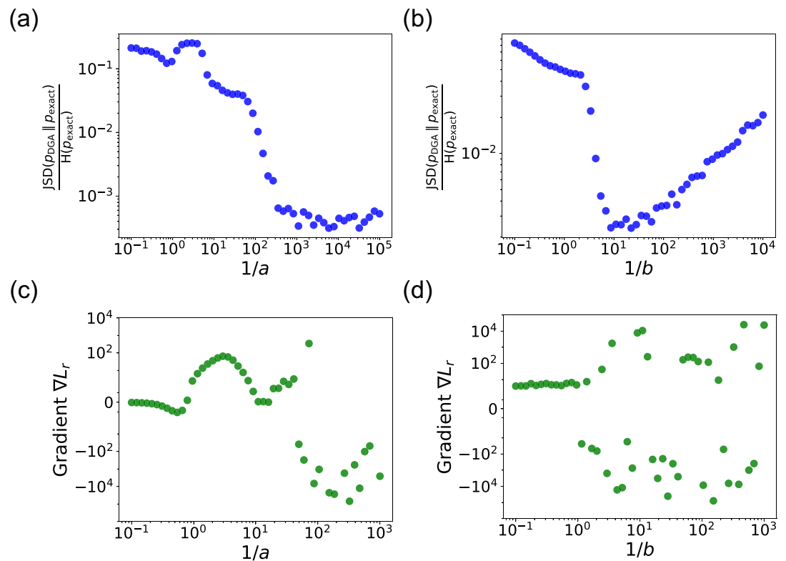
Appendix 1—figure 1. In panels (a) and (b), we plot the ratio of the Jensen–Shannon divergence \text{JSD}(p_{\text{DGA}} \| p_{\text{exact}}^{\text{ss}}) between the differentiable Gillespie PDF p_{\text{DGA}} and the exact steady-state PDF p_{\text{exact}}^{\text{ss}} , and the Shannon entropy H(p_{\text{exact}}^{\text{ss}}) of the exact steady-state PDF, as a function of the two sharpness parameters 1/a and 1/b . In panel (a), 1/b = 20 ; in panel (b), 1/a = 200 . The simulation time is set to 10. In panels (c) and (d), for these same values, we show the gradient \nabla L_r of the loss function L with respect to the parameter r near the true parameter values. In all the plots, the values of the rates are: k_{\text{on}}^R = 0.5 , k_{\text{off}}^R = 1 , r = 10 , and \gamma = 1 . 5000 trajectories are used to obtain the PDFs, while 200 trajectories are used to obtain the gradients.
