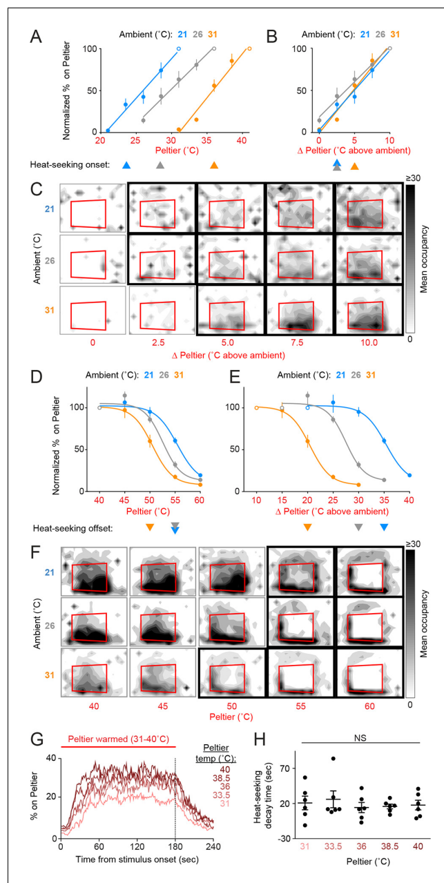
Figure 2. Mosquitoes thermotax to relative warmth and avoid both relative cooling and stimuli exceeding host body temperature. (A–F) Heat-seeking at different ambient temperatures ( n = 5 –6 trials per condition): 21°C (blue), 26°C (gray), 31°C (orange). Data in A, B, D, and E are plotted as mean \pm s.e.m. (A, D) Percent of mosquitoes on Peltier during seconds 90–180 of stimuli of indicated temperature, normalized to stimulus 10°C above ambient (A, open circle) or 40°C stimulus (D, open circle). (B, E) Same data as in (A) and (D), respectively, plotted using differential between ambient and Peltier temperature. For each ambient temperature, arrowheads indicate the lowest temperature stimulus found to elicit a significant increase in heat-seeking compared to an ambient temperature stimulus (A, B) or a reduction in heat-seeking compared to a 40°C stimulus (D, E) ( p < 0.05 ; repeated-measures ANOVA with Bonferroni correction). For each ambient temperature, linear regressions (A, B, 21°C: 10.6/^{\circ}\text{C} , R^2 = 0.98 , 26°C: 12/^{\circ}\text{C} , R^2 = 0.99 , 31°C: 9.5/^{\circ}\text{C} , R^2 = 0.97 ) or variable slope sigmoidal dose–response curves (D, E, 21°C: \text{IC}_{50} = 55.4^{\circ}\text{C} , R^2 = 0.87 , 26°C: \text{IC}_{50} = 52.5^{\circ}\text{C} , R^2 = 0.92 , 31°C: \text{IC}_{50} = 50.5^{\circ}\text{C} , R^2 = 0.91 ) are plotted. (C, F) Heat maps showing mean mosquito occupancy on the Peltier (red square) and surrounding area, during seconds 90–180 of each stimulus period. Bold borders indicate stimuli with responses significantly different from an ambient-temperature stimulus (C) in (A, B), or significantly different from a 40°C stimulus (F) in (D, E) ( p < 0.05 ; repeated-measures ANOVA with Bonferroni correction). (G, H) Analysis of mosquito responses to cooling from Figure 2 continued on next page
