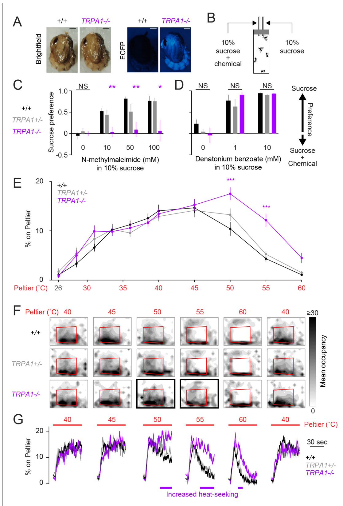
Figure 3. AegTRPA1 -/- mutants fail to avoid a chemical irritant and high-temperature stimuli. (A) Representative bright field (left) and fluorescence (right) images of wild-type and AegTRPA1 -/- female pupae marked by ubiquitous expression of enhanced cyan fluorescent protein (ECFP). Scale bars: 0.5 mm. (B) Schematic of capillary feeding (CAFE) assay. (C,D) Sucrose preference over sucrose containing the indicated concentration of N- Figure 3 continued on next page
