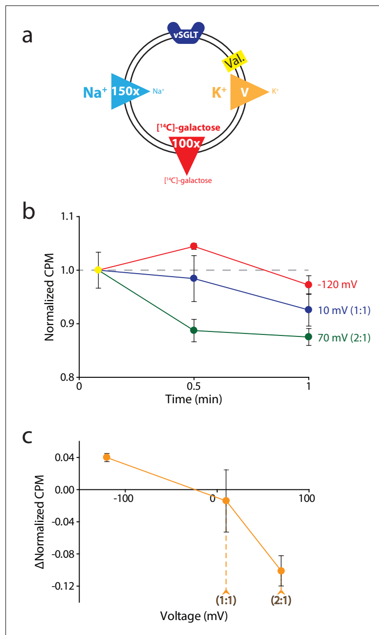
Figure 5. Reversal potential for vSGLT transport indicates a 1:1 coupling stoichiometry. (a) Schematic describing experimental conditions as in Figure 2a. , except with an outwardly directed [ 14 C]-galactose gradient instead of succinate. (b) Internalized [ 14 C]-galactose measured over time in the presence of three different voltages: −120 mV (red), 10 mV (blue), and 70 mV (green). The exact buffer conditions used in this experiment are detailed in Supplementary file 1. (c) Voltage-ΔCPM plot of the data in part (b). ΔCPM was calculated by subtracting the CPM values at 30 s from the normalized y-intercept. Numbers in parentheses represent coupling stoichiometry (Na + : galactose) for each membrane potential. Triplicate datasets are shown and the error bars represent S.E.M. This experiment was reproduced on two separate occasions.
