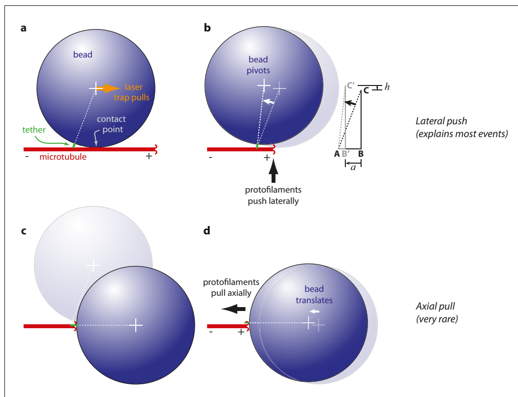
Figure 3. Proposed mechanisms underlying conformational wave-driven bead movement in the assay. (a) Initially, when a bead is placed under tension it rests against the microtubule wall at a secondary contact point. (b) In the lateral push scenario, the curling protofilaments push laterally against the secondary contact point, causing the bead to pivot about the base of the tether. Lateral deflections from the protofilaments, h , produce larger axial displacements of the bead, a . If A is the tether point and B is the point of bead-microtubule contact and C is the bead center, then ABC defines a right triangle and the amount of leverage is given by the ratio of sides BC/AB. The predicted leverage for 900 nm diameter beads attached via 36 nm tethers is a \cdot h^{-1} = 2.4 . (c) In the axial pull scenario, the microtubule first disassembles past the secondary contact point, allowing the bead to rotate under laser trap tension into an end-on configuration relative to the microtubule tip. (d) Then the working stroke occurs when curling protofilaments encounter the tether and pull axially on the bead.
