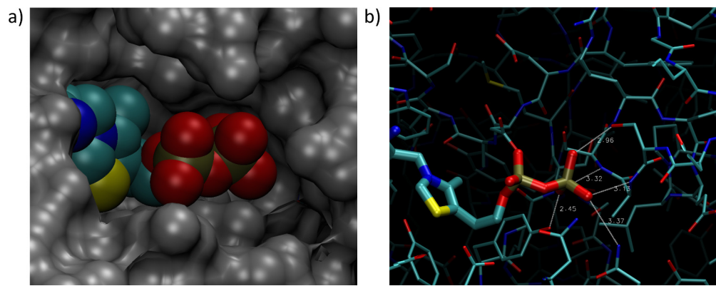
Appendix 1—figure 1. Thiamin diphosphate (ThDP) from the Mycoplasma hyorhinis Cypl crystal structure (pdb: 3EKI) overlaid onto the crystal structure of MG289 (pdb: 3MYU). (Structures aligned using STAMP (Russell and Barton, 1992) in VMD (Humphrey et al., 1996; Eargle et al., 2006).) a): Space-filling view, with MG289 in gray and ThDP in color. The pyrophosphate tail of ThDP from the Cypl structure would have an appropriate cavity in MG289 as well. b): Visualization of hydrogen bonds for the same alignment. All possible hydrogen bonds are shown between potential donor and acceptor heavy atoms within 3.5 Å or less of each other. Even in the absence of the residues involved in pyrophosphate binding in Cypl (Sippel et al., 2009), the alignment suggests other side group and backbone interactions could still allow for pyrophosphate binding.
