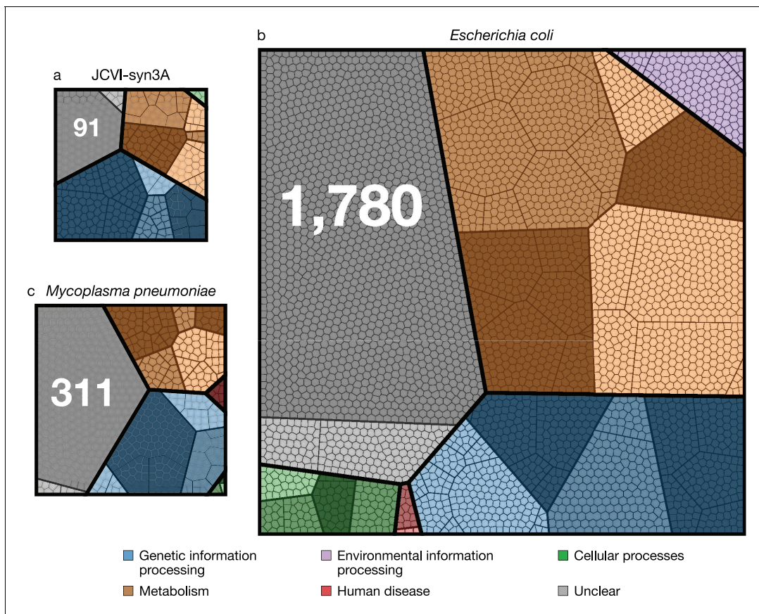
Figure 1. Comparison of protein coding genes in the genomes of JCVI-syn3A (NCBI GenBank: https://www.ncbi.nlm.nih.gov/nuccore/CP016816.2 (Glass, 2017)), M. pneumoniae (NCBI GenBank: https://www.ncbi.nlm.nih.gov/nuccore/U00089.2 (Himmelreich et al., 2014)), and E. coli (NCBI GenBank: https://www.ncbi.nlm.nih.gov/nuccore/NC_012967.1 (Jeong et al., 2017)) with 452, 688, and 4637 coding genes, respectively. Each color represents a primary functional class, each contiguous shaded region corresponds to a secondary functional class, within each of the shaded regions the bold lines separate tertiary functional classes, finally each polygonal cell represents a single gene. The functional class hierarchy is presented in Supplementary file 1A . The ratio of metabolic to genetic information processing genes—0.67, 0.79, and 2.23 respectively—is smallest for JCVI-syn3A. The JCVI-syn3A genome contains both the smallest absolute number of genes of unclear function and the smallest percentage, 91 (20%), compared to M. pneumoniae with 311 (45%) and E. coli with 1780 (38%).
