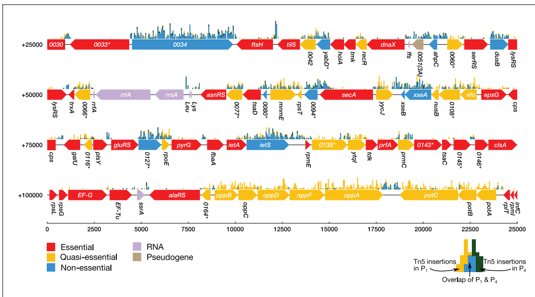
Figure 2. Classification of gene essentiality from transposon insertion data using a Poisson mixture model for a representative region of the JCVI-syn3A genome. Coding regions are colored by their predicted class: red (essential), yellow (quasi-essential), blue (non-essential). Lavender regions denote RNA and light brown regions are pseudogenes. The distributions of transposon insertions in passage 1 and passage 4 are represented by yellow and dark green histograms, respectively (bin size of 50 bp). The overlap of the two histograms is highlighted in blue. When a common gene name is not available, the four-digit locus tag for JCVI-syn1.0 is used instead. Locus number identifiers with the (3A) suffix represent newly identified open reading frames in JCVI-syn3A which are missing from the JCVI-syn1.0 annotation. Asterisks mark genes with unknown functionality.
