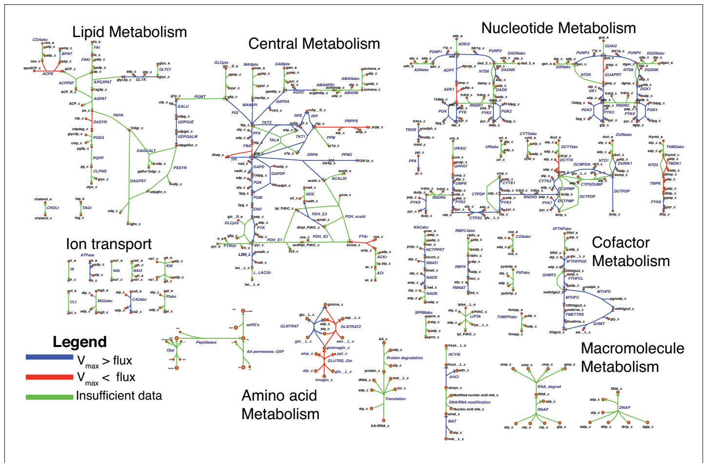
Figure 15. Comparison of FBA steady-state fluxes \nu to maximal fluxes V_{max} obtained from protein abundances and turnover numbers from BRENDA and the literature. Map components and labels as in Figure 5 , with reaction highlighting and gene loci/gene-protein-reaction rules omitted. Each edge is colored according to the ratio between V_{max} and \nu : Blue indicates V_{max} > \nu , red indicates V_{max} < \nu and green indicates that no V_{max} could be obtained (because of either missing turnover number or missing protein abundance; or because reaction is not enzymatic to begin with). The online version of this article includes the following figure supplement(s) for figure 15:
