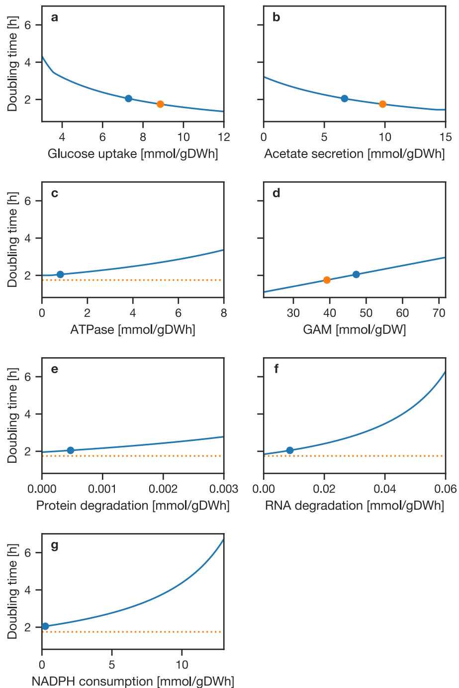
Appendix 1—figure 2. Sensitivity analysis of model doubling time with respect to model constraints. In each panel, the stated parameter was varied over the indicated range and the model doubling time calculated while keeping all other constraints constant. (A:) Maximal glucose uptake. (B:) Maximal acetate secretion. (C:) ATPase ATP cost. D: GAM ATP cost. (E:) Protein degradation rate. (F:) RNA degradation rate. (G:) Imposed NADPH consumption. The blue circle marks the value used in the FBA model and resulting doubling time; the orange circle indicates the parameter that would yield the experimental doubling time. If there is no value of the parameter which would yield the experimental doubling time, a horizontal line is plotted.
