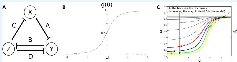
Appendix 1—figure 6. Connectionist AC/DC circuit. (A) Regulatory structure and parameters of the simulated AD/DC circuit. Nodes represent genes and their transcription-factor products. T-bars represent repressive regulatory interactions. All genes are constitutively activated. (B) Sigmoidal regulation-expression function used for the simulations ( Equation 31 ). (C) The number of steady states in the connectionist AD/DC circuit, can be one (black curves), or three (coloured curves) depending on the strength of the back reaction.
