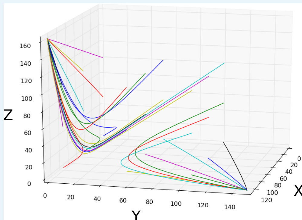
Appendix 1—figure 5. Bistability: simulation of the bistable dynamical regime. Trajectories with varying initial conditions (coloured curves) are shown to converge towards the two point attractors. This circuit was simulated using the connectionist formulation given by Equation 33 , and the parameter values shown in Appendix 1—table 3 .
