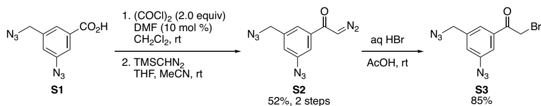
Scheme 1. Synthesis of compounds S1 - S3.
