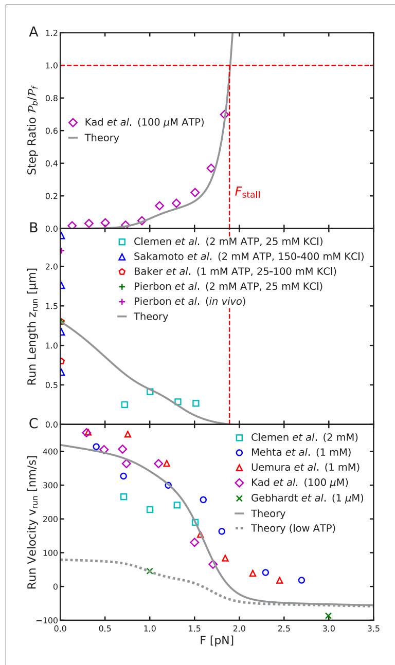
Figure 8. Load-dependent aspects of myosin V dynamics. (A) Backward-to-forward step ratio \mathcal{P}_b/\mathcal{P}_f ; (B) mean run length z_{run} ; (C) mean run velocity v_{run} . Analytical theory results are drawn as curves, experimental results as symbols. The legend symbols are the same as those in Hinczewski et al. (2013), for ease of comparison, but the theory curves have been updated.
