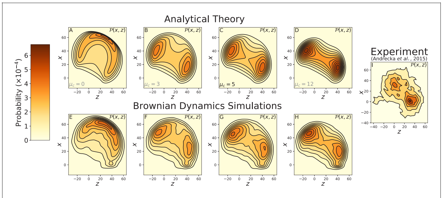
Figure 3. Contours of the myosin V free head position distribution \mathcal{P}(\mathbf{r}) projected onto the z-x plane. Top row: theoretical predictions for (A) free diffusion ( \mu_c = 0 ) and (B–D) constrained diffusion with inter-leg constraint strength (B) \mu_c = 3 , (C) \mu_c = 5 , and (D) \mu_c = 12 . Bottom row: the corresponding contours measured from Brownian dynamics simulations, with inter-leg constraint strength (E) \mu_c = 0 , (F) \mu_c = 3 , (G) \mu_c = 5 , and (H) \mu_c = 12 . (I) Experimental measurements of the diffusion by Andrecka et al. (2015) . Adding an inter-leg constraint potential produces a multi-peaked diffusion pattern. The heights of the peaks are similar to the experimental measurements for 3 \lesssim \mu_c \lesssim 12 . Note that the x = 0 axis in the experimental data corresponds to the position of the gold bead attached to the myosin head when the head is bound to actin. Given the \sim 5 nm size of the head and \sim 10 nm radius of the bead, this accounts for the approximately 15 nm vertical shift between the theoretical/simulation distributions and experiment. In the former the x = 0 axis corresponds to the top of the actin filament (where the bound head is attached).
