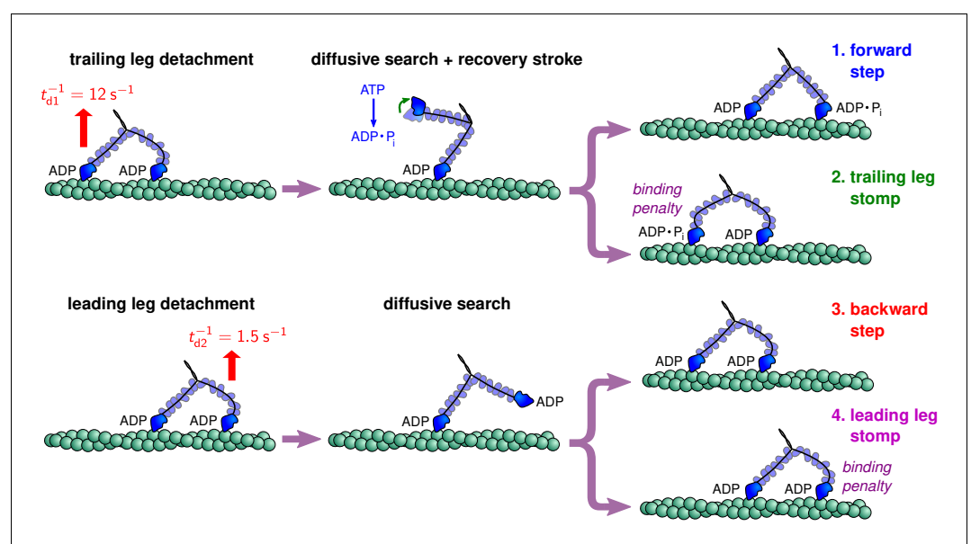
Figure 2. Myosin V kinetic pathways.
