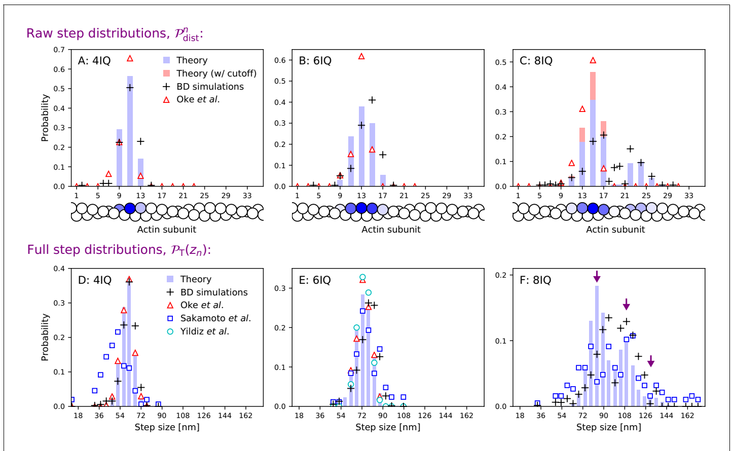
Figure 4. Step size distributions for myosin V and mutants with altered leg length. Top row: raw step distributions for (A) the 4IQ mutant, (B) the 6IQ wild-type, and (C) the 8IQ mutant. Bottom row: full (convolved) step distributions for (D) the 4IQ mutant, (E) the 6IQ wild-type, and (F) the 8IQ mutant, with three theoretical peak locations indicated by arrows. Theoretical distributions are shown as histograms with Brownian dynamics simulations and experimental data from Oke et al. (2010) , Sakamoto et al. (2005) , and Yildiz et al. (2003) indicated by symbols. The raw data from Oke et al. (2010) is convolved and binned in the bottom row. Since the imaging methods used in this experiment did not resolve large steps taken by the 8IQ mutant, in panel C we show an alternative theory (in red) with a cutoff where only small steps are allowed. The actin monomers drawn below the top row are shaded according to this analytical theory results, with the darkest color normalized to the peak of the distribution.
