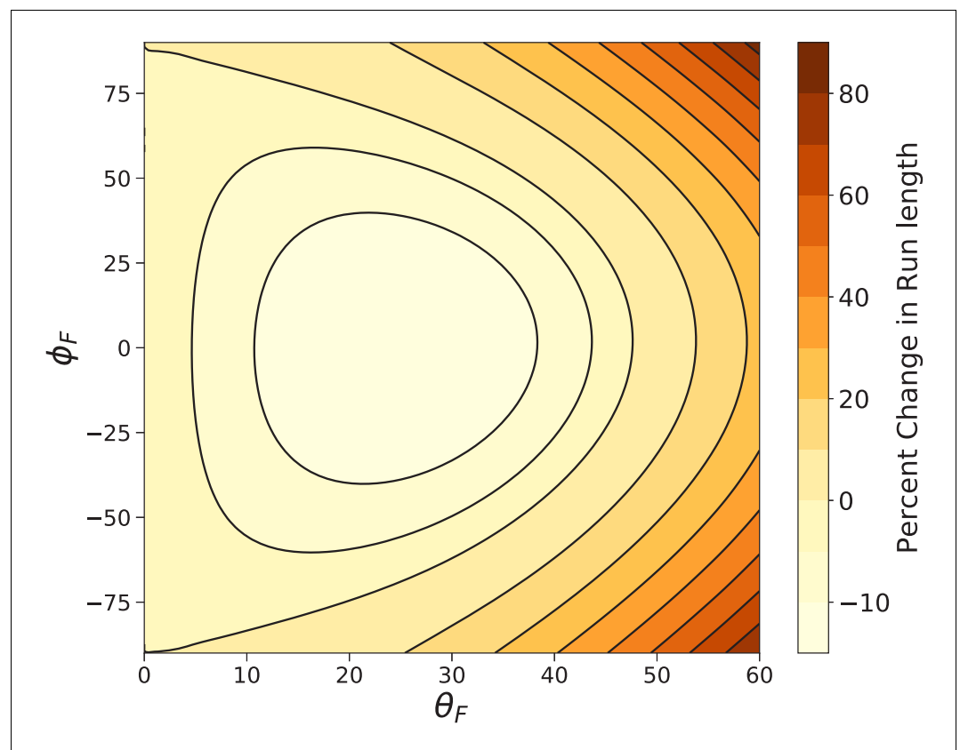
Figure 9. Myosin V run length under off-axis forces. Shown is the percent change in run length from that under backward force z_{\text{run}}(\theta_F, \phi_F) / z_{\text{run}}(0, 0) - 1 computed using Equation 9 . In the worst case (\theta_F \approx 20^\circ, \phi_F = 0) the run length is decreased by \sim 15\% . The run length most dramatically increases under fully off-axis forces (\theta_F > 0, \phi_F = \pm 90^\circ) .
