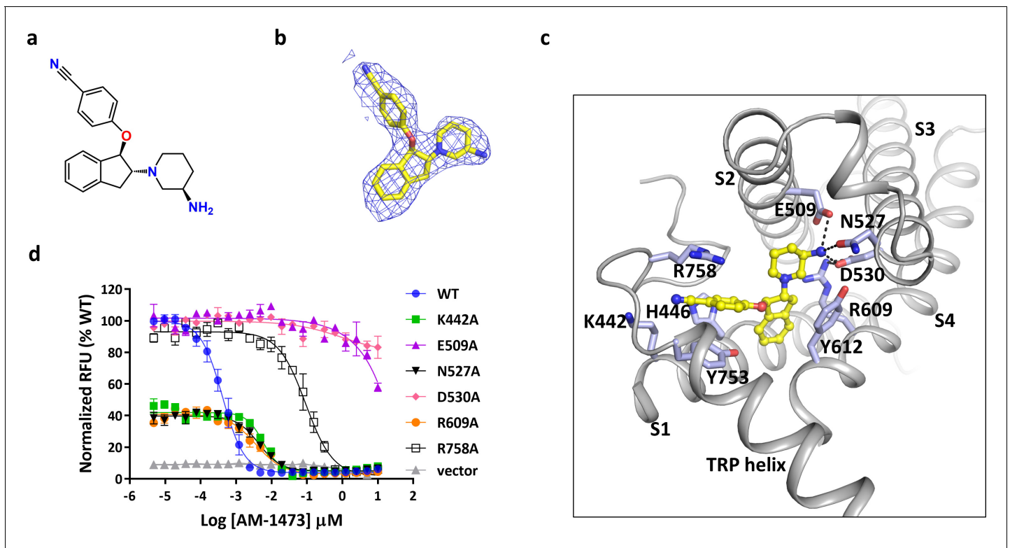
Figure 2. Binding of antagonist to TRPC6. (a) Chemical structure of the antagonist AM-1473. (b) Stick model of the antagonist bound to the TRPC6 protein, with EM density shown as a blue mesh. (c) Close-up view of the antagonist-binding site. Residues within van der Waals distances are shown in light blue sticks. Hydrogen bonds are shown in black dashed lines. (d) Dose-response curves for TRPC6 inhibition of wild-type and mutant TRPC6 channels replacing residues that interact with the antagonist.
