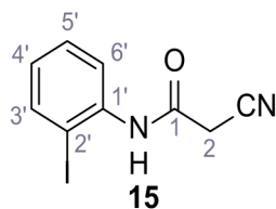
Chemical structure 16. 2-Cyano-N-(2-iodophenyl)acetamide (15).
