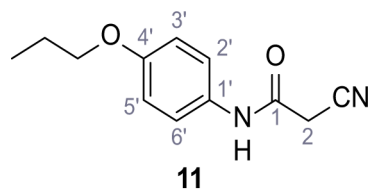
Chemical structure 12. 2-Cyano-N-(4-propoxyphenyl)acetamide (11).
