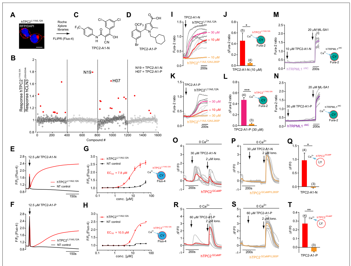
Figure 1. Identification of novel small molecule agonists of TPC2. (A) The chemical screening was performed using cells stably expressing human TPC2 re-routed to the plasma membrane (hTPC2 L11A/L12A ) and loaded with the fluorescent Ca 2+ indicator, Fluo-4 (CY = cytosol). For counter-screening, a stable cell line expressing cell surface human CLN3 (hCLN3 L253A/I254A ) was used. (B) A library comprising 80,000 compounds was screened. Shown are the primary screen results of four plates (with 384 compounds, each) where the response to a given compound in cells expressing hTPC2 L11A/L12A is expressed relative to that in cells expressing hCLN3 L253A/I254A . Primary hits are shown as red spots. Subsequent confirmatory and follow-up assays led to the identification of the two hit compounds, N19 (TPC2-A1-N) and H07 (TPC2-A1-P). (C–D) Figures of TPC2-A1-N and TPC2-A1-P. (E–F) Representative FLIPR-generated Ca 2+ signals (Fluo-4) in TPC2 L11A/L12A -expressing cells (red lines) or non-transfected (NT) control cells (black) after addition of TPC2-A1-N (E) or TPC2-A1-P (F). (G–H) Concentration-effect relationships for Ca 2+ increases (Fluo-4) in response to different concentrations of TPC2-A1-N (G) and TPC2-A1-P (H). Each concentration was tested in duplicates in two to four independent experiments, each. (I) Representative Ca 2+ signals recorded from HeLa cells loaded with the ratiometric Ca 2+ indicator, Fura-2 and stimulated with the indicated concentration of TPC2-A1-N. Cells were transiently transfected with plasma-membrane-targeted human TPC2 (hTPC2 L11A/L12A ) or a pore dead mutant (TPC2 L11A/L12A/L265P ). Colored lines represent the mean response from a population of cells. Traces in grey represent responses of single cells. (J) Statistical analysis of the maximal change in Fura-2 ratio (mean ± SEM) with the number of independent transfections in parentheses. An unpaired t-test was applied. *p<0.05. (K–L) Similar to I and J except that cells were stimulated with TPC2-A1-P. ***p<0.001. Traces in grey represent single cells responding to TPC2-A1-P. (M–N) Representative Ca 2+ signals recorded from HeLa cells transiently transfected with human TRPML1 ΔNC . Cells were sequentially stimulated with TPC2-A1-N (M) or TPC2-A1-P (N) and the TRPML agonist ML-SA1. (O–T) Ca 2+ signals recorded from HeLa cells transiently transfected with GCaMP6(s) fused to human TPC2 (hTPC2 GCaMP ) or a pore-dead mutant (hTPC2 GCaMP/L265P ). Cells were sequentially stimulated with TPC2-A1-N (O and P) or TPC2-A1-P (R and S) and the Ca 2+ ionophore, ionomycin in the absence of extracellular Ca 2+ . Statistical analysis of the change in fluorescence intensity (mean ± SEM; Q and T). An unpaired t-test was applied. *p<0.05 and **p<0.01. CY = cytosol, LY = lysosome.
