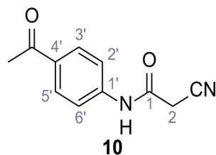
Chemical structure 11. N-(4-Acetylphenyl)-2-cyanoacetamide (10).
