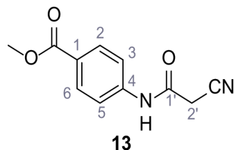
Chemical structure 14. Methyl 4-(2-cyanoacetamido)benzoate (13).
