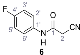
Chemical structure 7. 2-Cyano- N -(4-fluorophenyl)acetamide (6).
