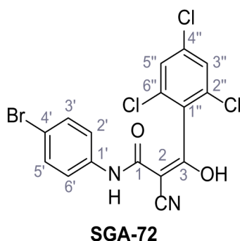
Chemical structure 48. N-(4-Bromophenyl)-2-cyano-3-hydroxy-3-(2,4,6-trichlorophenyl)acrylamide – SGA-72.
