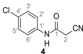
Chemical structure 5. N-(4-Chlorophenyl)-2-cyanoacetamide (4).
