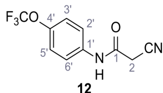
Chemical structure 13. 2-Cyano-N-(4-(trifluoromethoxy)phenyl)acetamide (12).
