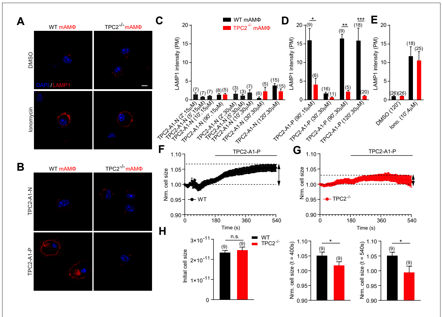
Figure 5. TPC2 agonists differentially affect lysosomal exocytosis. (A–B) Representative images of LAMP1 translocation assay using murine wild-type and TPC2 KO alveolar macrophages. Shown are results obtained after 120 min treatment with either DMSO, TPC2-A1-P (30 μM) or TPC2-A1-N (30 μM), or 10 min treatment with ionomycin (4 μM). (C–E) Statistical analysis of experiments as shown in A and B at different compound concentrations and incubation times as indicated. Shown are mean values ± SEM. ** p < 0.01 , and *** p < 0.001 , using two-way ANOVA followed by Bonferroni's post hoc test. (F–G) Electrophysiological measurements of membrane capacitance via the whole-cell patch-clamp technique as an estimate of cell size (in picofarad [pF]) were used to record fusion of vesicles of primary alveolar macrophages isolated from WT (black, n = 9 , F) or TPC2 KO (red, n = 9 , G) mice. The normalized, averaged cell size was plotted versus time of the experiment. TPC2-A1-P (30 μM) was applied at 180 s until the end of the experiment indicated by the black bar. Data are shown as mean ± SEM. (H) Bar graphs show mean cell sizes at different time points. The initial cell size was measured immediately after whole cell break in pF and was used for normalization (left panel). Statistical analysis at 400 s (middle panel) and at 540 s (right panel). * p < 0.05 , unpaired student's t-test.
