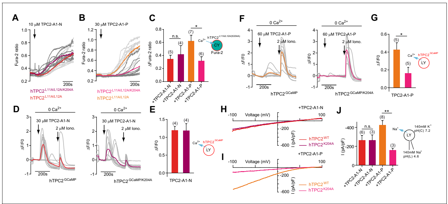
Figure 3. TPC2 agonists activate TPC2 through distinct sites. (A–B) Representative Ca 2+ signals recorded from Fura-2-loaded HeLa cells (n = 10, each) stimulated with the indicated concentration of TPC2-A1-N or -P. Cells were transiently transfected with plasma membrane targeted human TPC2 (hTPC2 L11A/L12A ) or the PI(3,5)P 2 -insensitive mutant (TPC2 L11A/L12A/K204A ). (C) Statistical analysis of the maximal change in Fura-2 ratio (mean ± SEM) with the number of independent transfections in parentheses. An unpaired t-test was applied. *p<0.05. (D–F) Representative Ca 2+ signals recorded from HeLa cells (n = 10, each) transiently transfected with GCaMP6(s) fused to wild-type TPC2 (TPC2 GCaMP6(s) ) or the PI(3,5)P 2 -insensitive mutant (TPC2 GCaMP6(s)/K204A ). Cells were sequentially stimulated with TPC2-A1-N or -P and the Ca 2+ ionophore ionomycin in the absence of extracellular Ca 2+ . (E–G) Statistical analysis of the change in fluorescence intensity (mean ± SEM) of experiments as shown in D and F. An unpaired t-test was applied. *p<0.05. (H–I) Representative TPC2-A1-N or -P-evoked currents from enlarged endo-lysosomes isolated from HEK293 cells transiently expressing human TPC2 (hTPC2) or the PI(3,5)P 2 -insensitive mutant, (hTPC2 K204A ). Currents were obtained before and after addition of 10 μM TPC2-A1-N or -P. Recordings were carried out using standard bath and pipette solutions and applying ramp protocols (–100 mV to +100 mV over 500 ms) every 5 s at a holding potential of –60 mV. (J) Statistical analysis of current densities (mean ± SEM) recorded at –100 mV for endo-lysosomes expressing TPC2 or TPC2 K204A using TPC2-A1-N or TPC2-A1-P to activate, respectively. *p<0.05 and **p<0.01, using one-way ANOVA followed by Tukey’s post hoc test. The online version of this article includes the following source data for figure 3:
