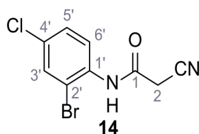
Chemical structure 15. N-(2-Bromo-4-chlorophenyl)-2-cyanoacetamide (14).
