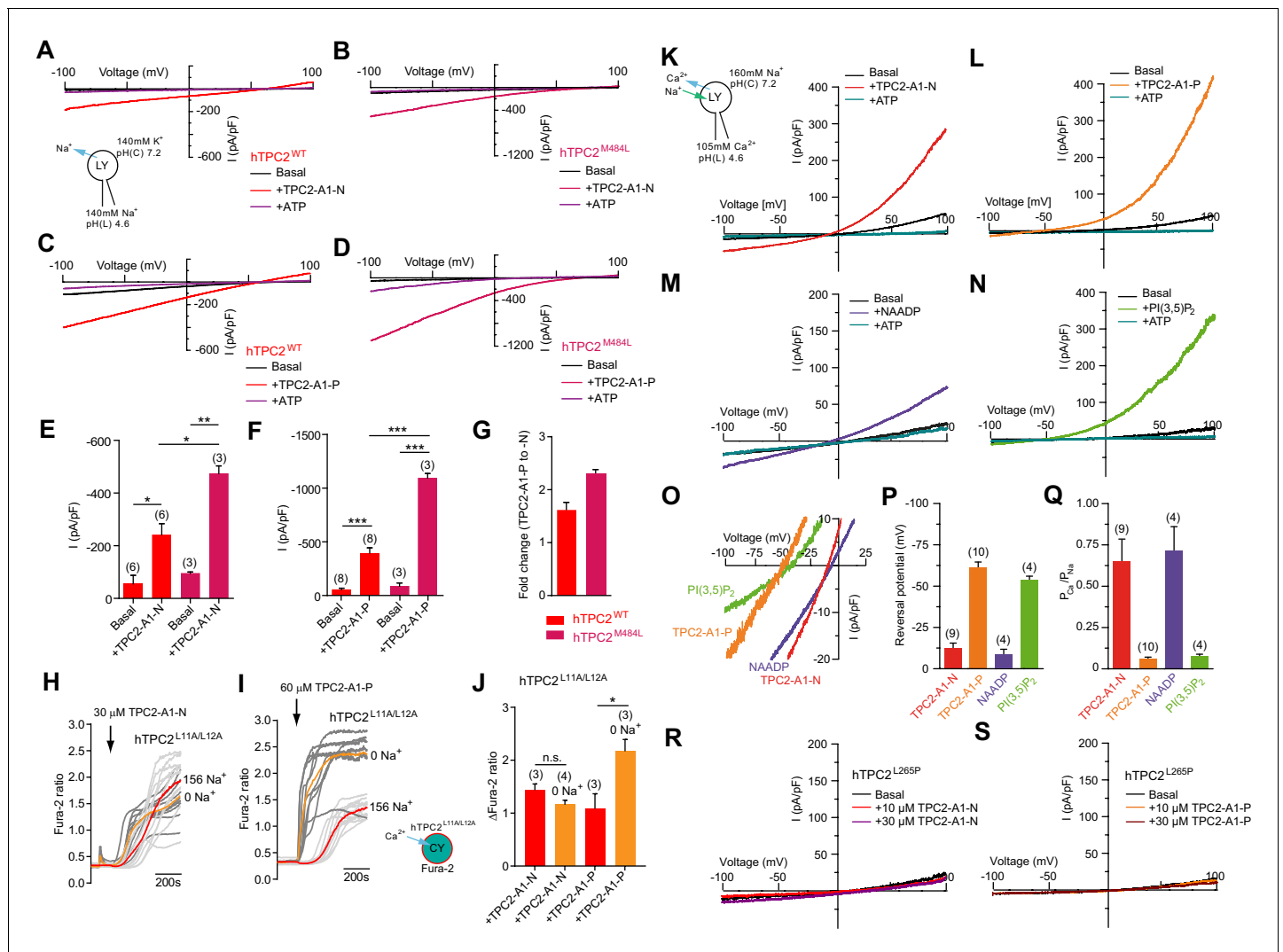
Figure 2. TPC2 agonists alter \text{Ca}^{2+}/\text{Na}^{+} permeability of TPC2. (A–B) Representative TPC2-A1-N-evoked currents from enlarged endo-lysosomes isolated from HEK293 cells transiently expressing human TPC2 (hTPC2) (A) or a gain-of-function variant, (hTPC2 M484L ) (B). Currents were obtained before and after addition of 10 \mu\text{M} TPC2-A1-N in the absence or presence of 1 mM ATP. Recordings were carried out using standard bath and pipette solutions and applying ramp protocols (–100 mV to +100 mV over 500 ms) every 5 s at a holding potential of –60 mV. (C–D) Similar to A and B except that TPC2-A1-P (10 \mu\text{M} ) was used. (E–G) Statistical analysis of current densities (mean \pm SEM) recorded at –100 mV for endo-lysosomes expressing TPC2 or TPC2 M484L for TPC2-A1-N (E) and TPC2-A1-P (F), and the fold-change in current evoked by TPC2-A1-P versus TPC2-A1-N in the two variants (G). Red bars are WT and maroon bars are mutant. An unpaired t-test was applied. * p < 0.05 , ** p < 0.01 , and *** p < 0.001 ( n > 10 endo-lysosomes per condition). (H–I) \text{Ca}^{2+} signals evoked by TPC2-A1-N (H) or TPC2-A1-P (I) in Fura-2-loaded HEK293 cells stably expressing hTPC2 L11A/L12A . Recordings (mean responses from three to four independent experiments) were obtained in standard or \text{Na}^{+} -free extracellular solution. (J) Statistical analysis of the maximal change in Fura-2 ratio (mean \pm SEM). An unpaired t-test was applied. * p < 0.05 . (K–N) Agonist-evoked cation currents from enlarged endo-lysosomes isolated from HEK293 cells stably expressing human TPC2 under bi-ionic conditions: 160 mM \text{Na}^{+} in the cytosol (bath) and 105 mM \text{Ca}^{2+} in the lumen (pipette). Representative current-voltage curves before and after stimulation with either 10 \mu\text{M} TPC2-A1-N (K), 10 \mu\text{M} TPC2-A1-P (L), 50 nM NAADP (4 recordings out of 8 attempts) (M), or 1 \mu\text{M} PI(3,5)P 2 (N). ATP (1 mM) was added at the end of each experiment. Recordings were carried out using ramp protocols (–100 mV to +100 mV over 500 ms) every 5 s at a holding potential of 0 mV. (O) Expanded views of K–N, showing the reversal potentials ( E_{\text{rev}} ) of currents evoked by the indicated agonist. (P–Q) Statistical analyses of E_{\text{rev}} (P) and the calculated relative cationic permeability ratios ( P_{\text{Ca}}/P_{\text{Na}} ) (Q). Shown are mean values \pm SEM. (R–S) Representative TPC2-A1-N- (R) or TPC2-A1-P- (S) evoked currents from endo-lysosomes isolated from HEK293 cells transiently expressing hTPC2 L265P under bi-ionic conditions.
