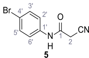
Chemical structure 6. N-(4-Bromophenyl)-2-cyanoacetamide (5).
