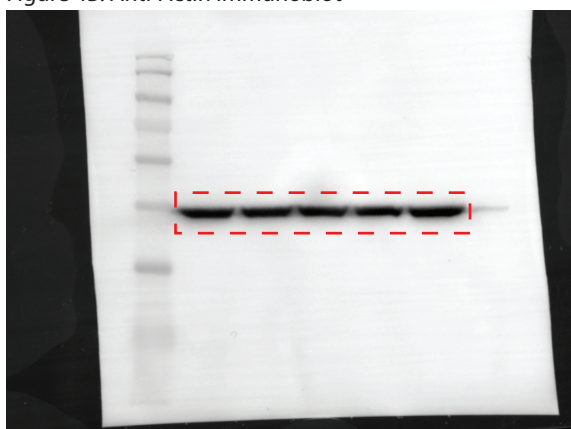
Figure 4B: Anti-Actin immunoblot
