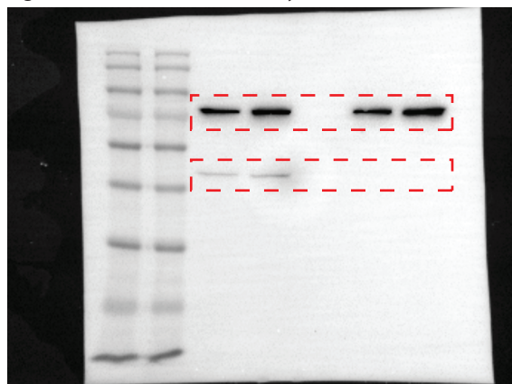
Figure 4B: Anti-GFP and Anti-Myc immunoblot
