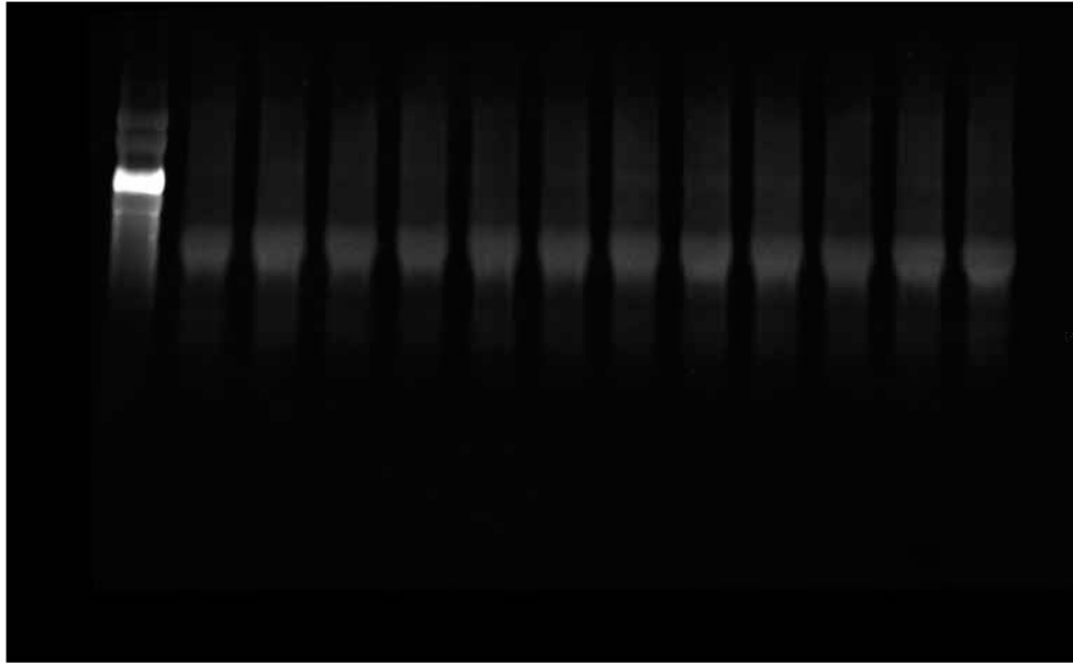
labelled northern, actin probe
