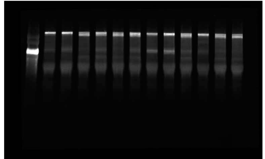
labelled northern, ITS1 probe
