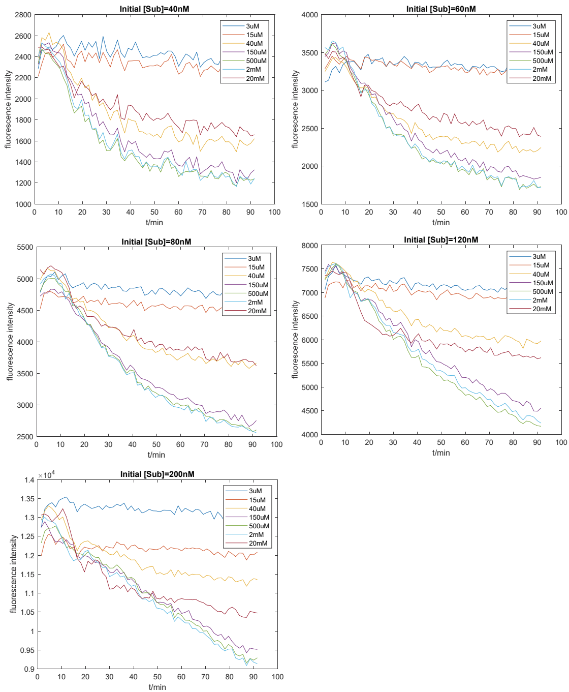
Source data related to figure 4B. Ubiquitylated cycB-iRFP (sub) at indicated concentrations was incubated with purified 26S proteasome in the presence of various concentrations of ATP-Mg 2+ . The fluorescence intensity from iRFP was monitored using a plate reader. Each trace is an average of three replica.
