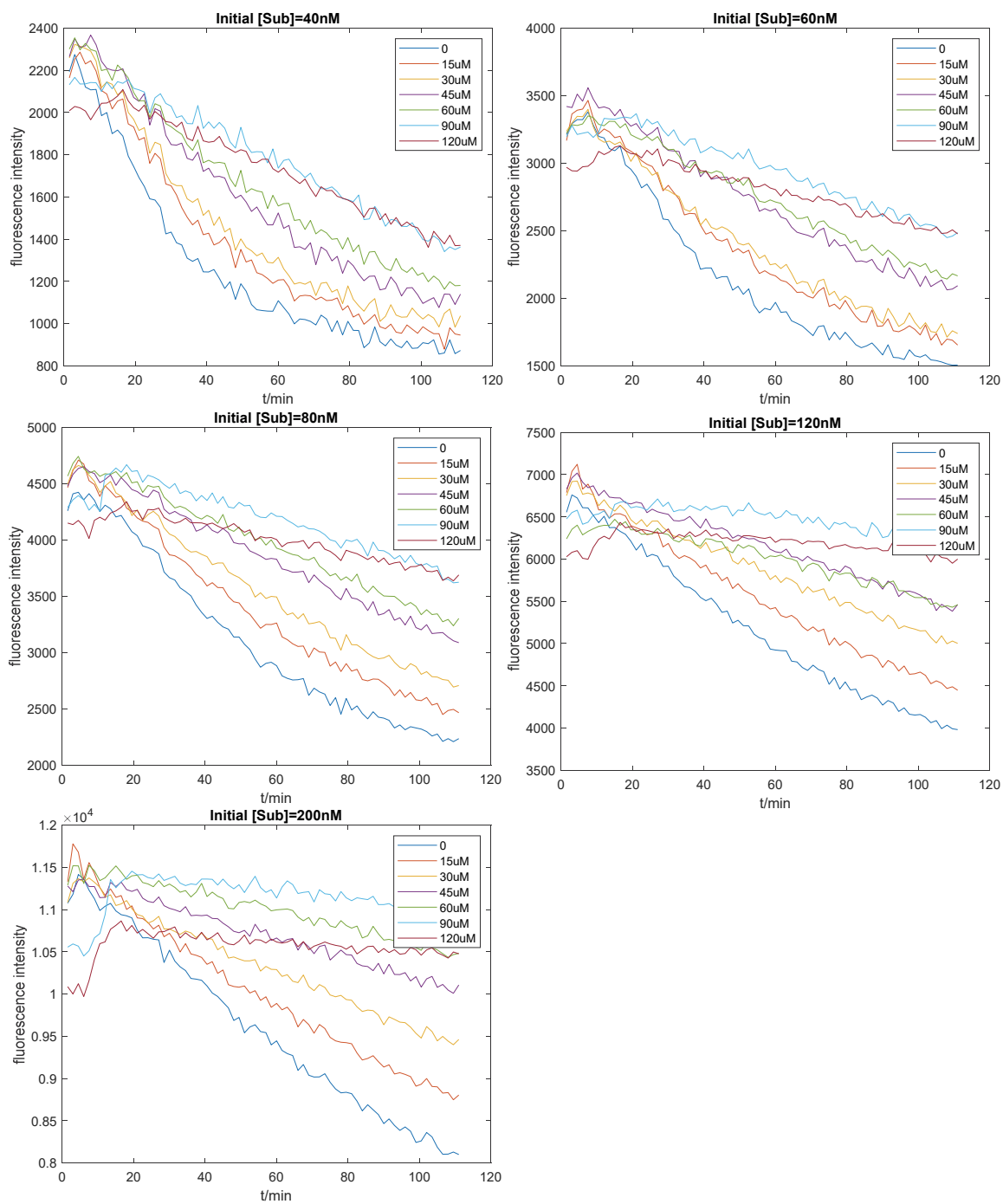
Source data related to figure 4C,D. Ubiquitylated cycB-iRFP (sub) at indicated concentrations was incubated with purified 26S proteasome in the presence of 500uM ATP plus various concentrations of ATP- \gamma S. The fluorescence intensity from iRFP was monitored using a plate reader. Each trace is an average of three replica.
