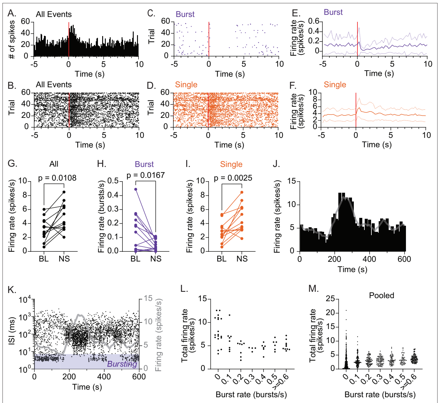
Figure 3. CRHP PVN neurons are constrained to low activity during rhythmic bursting. (A) Peristimulus time histogram (PSTH) for a representative single-unit responding to sciatic nerve stimulation (1.5 mA, 0.5 ms \times 5 pulses at 20 Hz, red line). (B–D) Raster plots for the unit shown in A for all spikes (B), bursts (C) and single spikes (SS) (D). (E, F) Summary time course for bursts (E) and SS (F). n=13 . (G–I) Summary changes in all spikes (G, paired t -test, n=13 , p=0.0108 ), bursts (H, paired t -test, n=13 , p=0.0167 ) and SS (I, paired t -test, n=13 , p=0.0025 ) before (baseline, BL) and after sciatic nerve stimulation (NS). (J, K) Time course of firing rate (J) and interspike interval (ISI) (K) for a representative single-unit during baseline recording. Gray lines are the running average (30 s) of firing rate. (L) The relationship between burst rate and total firing rate for the representative single-unit shown in J and K. For each time bin (10 s), total spike rate was plotted against burst rate. (M) Pooled data for all units ( n=18 ).
