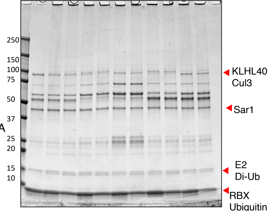
Colloidal Staining
