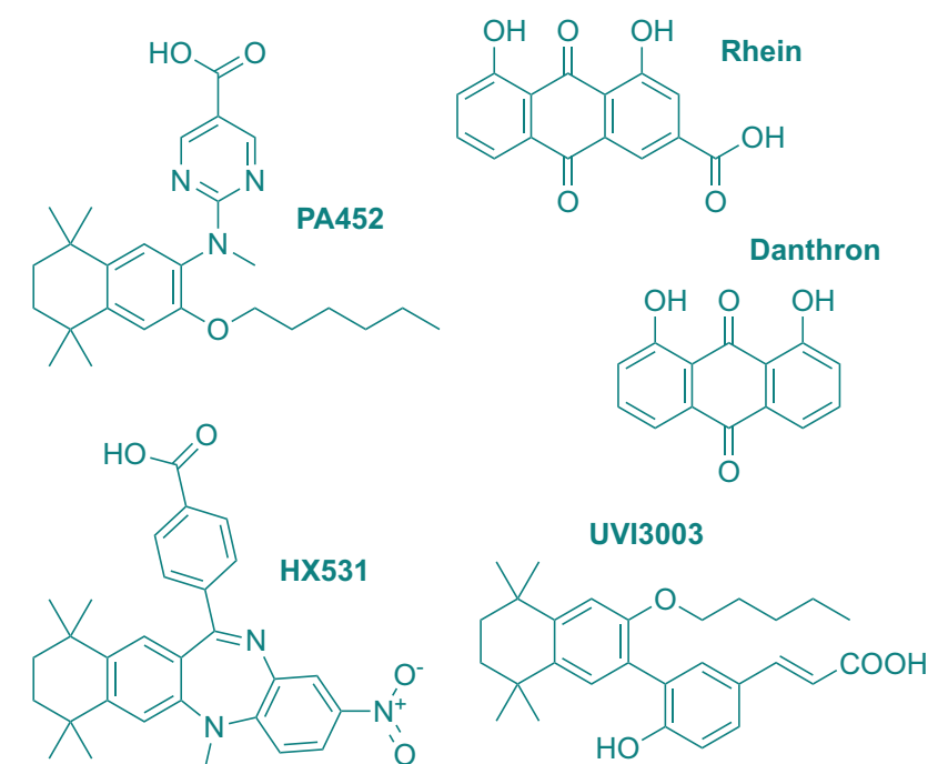
Figure 2. Retinoid X receptor alpha (RXR \alpha ) ligands used in this study. Grouped by pharmacological phenotype, the set includes ligands that classically activate (agonists) or block (antagonists) activation of RXR \alpha homodimers; a mixed activity modulator (LG100754) that antagonizes RXR \alpha homodimers and activates PPAR \gamma -RXR \alpha and RAR-RXR \alpha heterodimers; and two selective activators of Nurr1-RXR \alpha heterodimers (BRF110 and HX600).
