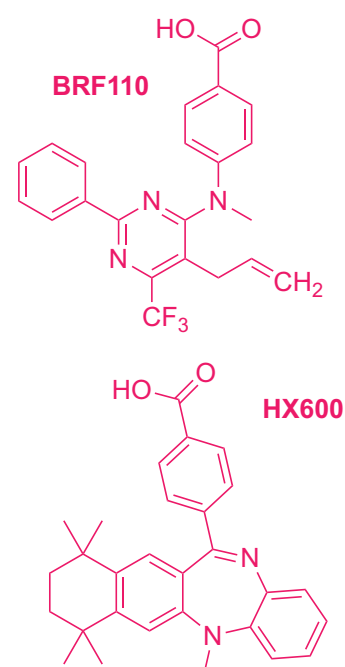
Figure 2. Retinoid X receptor alpha (RXR \alpha ) ligands used in this study. Grouped by pharmacological phenotype, the set includes ligands that classically activate (agonists) or block (antagonists) activation of RXR \alpha homodimers; a mixed activity modulator (LG100754) that antagonizes RXR \alpha homodimers and activates PPAR \gamma -RXR \alpha and RAR-RXR \alpha heterodimers; and two selective activators of Nurr1-RXR \alpha heterodimers (BRF110 and HX600).
