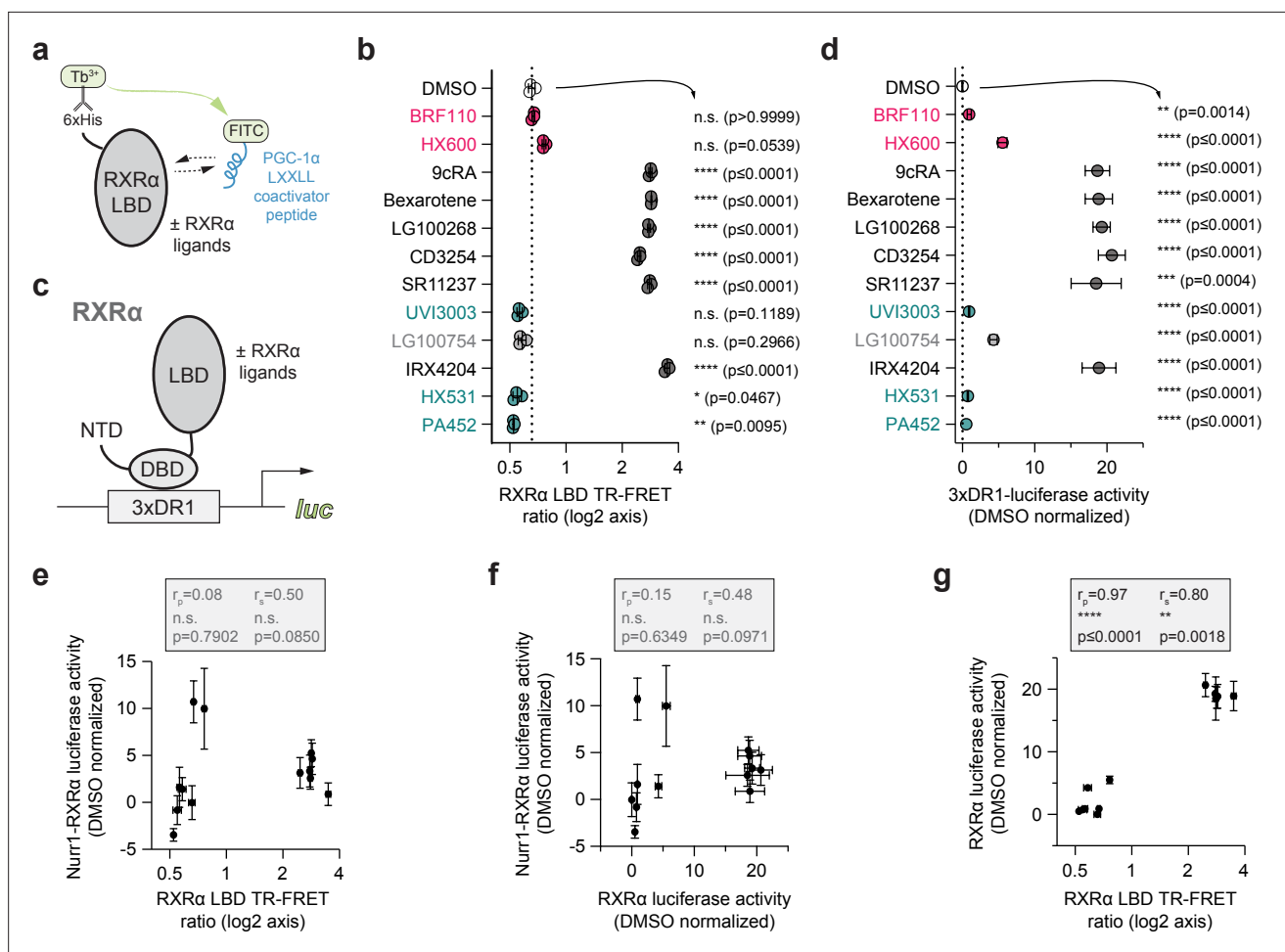
Figure 4. Compound profiling for pharmacological retinoid X receptor alpha (RXRα) agonism and correlation to Nurr1-RXRα agonism. (a) General scheme of the RXRα ligand-binding domain (LBD) time-resolved fluorescence resonance energy transfer (TR-FRET) coactivator peptide interaction assay. (b) TR-FRET ratio measured in the presence of DMSO (dotted line) or compound (2–4 μM); see Figure 4—source data 1 for data plotted. Data are normalized to DMSO control (n=3 biological replicates), represent the mean ± s.d., representative of two or more independent experiments. Statistical testing was performed and p-values were calculated using ordinary one-way ANOVA tests for multiple comparisons with Dunnett corrections relative to DMSO control treated condition. (c) General scheme of the RXRα/3xDR1-luciferase cellular transcriptional reporter assay. (d) RXRα/3xDR1-luciferase transcriptional reporter assay performed in HEK293T cells treated with compound (1 μM) or DMSO control (dotted line); see Figure 4—source data 2 for data plotted. Data normalized to DMSO (n=6 replicates), represent the mean ± s.d., and representative of two or more independent experiments. Statistical testing was performed and p-values were calculated using the Brown-Forsythe and Welch multiple comparisons test relative to DMSO control treated condition. (e) Correlation plot of RXRα LBD TR-FRET data vs. Nurr1-RXRα cellular transcription data. (f) Correlation plot of RXRα transcriptional reporter data vs. Nurr1-RXRα cellular transcription data. (g) Correlation plot of RXRα transcriptional reporter data vs. RXRα LBD TR-FRET data. Pearson ( r_p ) and Spearman ( r_s ) correlation coefficients and statistical significance testing are reported above the correlation plots.
