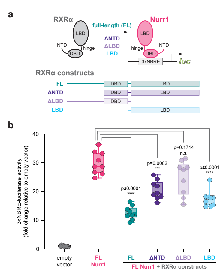
Figure 1. Contribution of retinoid X receptor alpha (RXRα) domains on repressing Nurr1 transcription. (a) General scheme of the cellular transcriptional reporter assay. (b) 3xNBRE-luciferase assay performed in SK-N-BE(2)-C cells; see Figure 1—source data 1 for data plotted. Data are normalized to empty vector control (n=9 replicates), shown as a box and whiskers plot with boundaries of the box representing the 25th percentile and the 75th percentile, and representative of two or more independent experiments. Statistical testing was performed and p-values were calculated using the Brown-Forsythe and Welch multiple comparisons test of the FL Nurr1 + RXRα constructs conditions relative to FL Nurr1 control condition.
