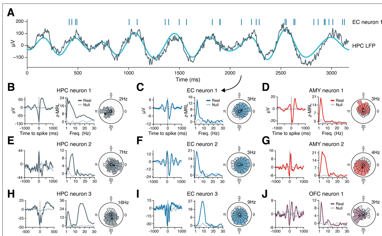
Figure 2. Example phase-locking to hippocampal oscillations. (A) Spikes from an EC neuron (top, vertical lines) are shown alongside local field potential (LFP) activity in the hippocampus during a slow theta oscillation (gray line = raw LFP, cyan line = 3 Hz–filtered LFP). Panel (C) shows phase-locking statistics for this neuron across the recording session. (B–J) Shown are nine neurons in the HPC (left column), EC (middle column), AMY (right column, top two rows), and OFC (right column, bottom row) that phase-locked to oscillatory signals in the hippocampus while subjects navigated through a virtual environment. The left subpanel for each neuron shows the mean hippocampal LFP centered on the time of each spike. The middle subpanel shows the phase-locking strength at each frequency relative to a null distribution of circularly shifted spikes. The right subpanel shows the spike–phase distribution at the maximum phase-locking frequency. Dark gray (HPC), blue (EC), red (AMY), and purple (OFC) lines correspond to true spike times, while light gray lines correspond to circularly shifted spike times from a single draw from the null distribution. HPC = hippocampus; EC = entorhinal cortex; AMY = amygdala; OFC = orbitofrontal cortex.
