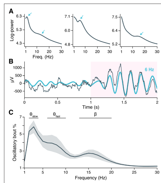
Figure 1. Neural oscillations in the hippocampus. (A) Spectral power across the recording session is shown for hippocampal local field potentials (LFPs) from three example subjects. Arrows indicate spectral peaks above the background 1/f spectrum. (B) A hippocampal LFP trace (gray line = raw LFP, cyan line = 6 Hz-filtered LFP) is shown immediately before and during a Better OSCillation (BOSC)-detected theta oscillation, highlighted in pink. (C) Mean \pm SEM percent time, across 28 subjects, that BOSC-detected oscillations were present in hippocampal LFPs at each frequency from 1 to 30 Hz.
