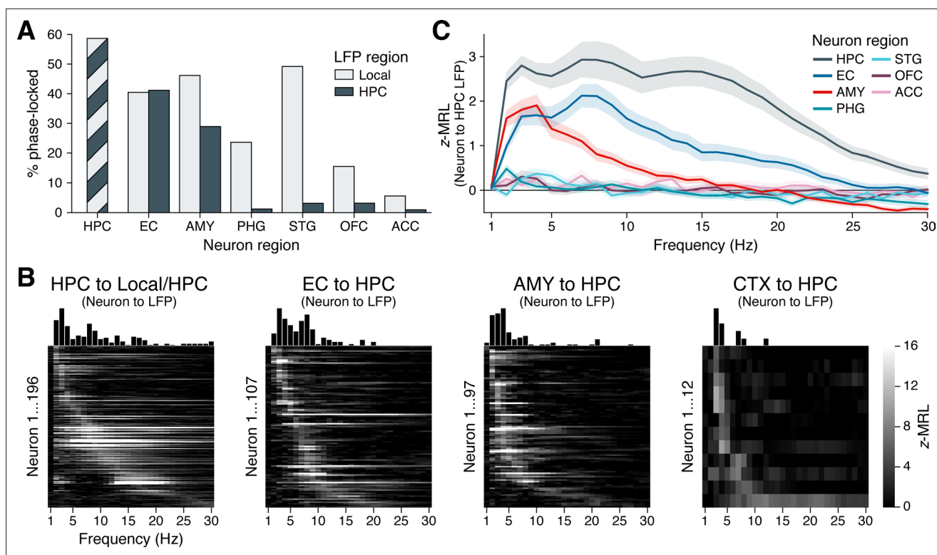
Figure 3. Phase-locking to hippocampal oscillations by region and frequency. (A) Bars show the percentage of neurons in each region that phase-locked to locally recorded local field potential (LFP) oscillations (light gray) and hippocampal LFP oscillations (dark gray). (Note that local and hippocampal LFP is identical for hippocampal neurons.) Phase-locking significance was set at false discovery rate (FDR)-corrected p < 0.05 within each bar group. (B) Heatmaps show the phase-locking strength (z-MRL; color scale intensity) by hippocampal LFP oscillation frequency (x-axis) for all significantly phase-locked neurons (y-axis; each row = one neuron) in the HPC, EC, AMY, and remaining regions (CTX), respectively. Neurons in each region are sorted from top to bottom by frequency of maximum phase-locking strength. Neurons depicted match the dark gray bars in (A) . (C) Mean \pm SEM phase-locking strength by hippocampal oscillation frequency is shown for all neurons in each region, regardless of their individual phase-locking significance as depicted in (A) and (B) . HPC = hippocampus; EC = entorhinal cortex; AMY = amygdala; PHG = parahippocampal gyrus; STG = superior temporal gyrus; OFC = orbitofrontal cortex; ACC = anterior cingulate cortex.
