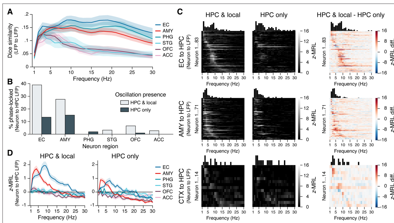
Figure 4. Phase-locking to hippocampal oscillations with and without co-occurring local oscillations. (A) Mean \pm SEM (across 28 subjects) Dice coefficient across subjects shows the percent overlap between oscillatory bouts in the hippocampus and in each extrahippocampal region. (B) Bars show the percentage of neurons in each region that phase-locked to hippocampal oscillations when local oscillations were present (light gray) or absent (dark gray). Phase-locking significance was set at false discovery rate (FDR)-corrected p < 0.05 within each bar group. (C) Heatmaps show the phase-locking strength by hippocampal LFP oscillation frequency for all significantly phase-locked neurons in the EC (top row), AMY (middle row), and remaining regions (CTX; bottom row), when hippocampal and local oscillations co-occurred (left column) versus when only hippocampal oscillations occurred (middle column). The right column shows the left column minus middle column values. Neurons in each region are sorted from top to bottom by frequency with the maximum phase-locking strength, and the sorting order is constant across columns within each row. Neurons depicted match the union of light gray and dark gray bars in (B) . (D) Phase-locking to the hippocampus is shown during co-occurring local and hippocampal oscillations (left) or only hippocampal oscillations (right). Each subpanel shows the mean \pm SEM (across 28 subjects) phase-locking strength by hippocampal oscillation frequency for all neurons in each region, regardless of their individual phase-locking significance as depicted in (B) and (C) . HPC = hippocampus; EC = entorhinal cortex; AMY = amygdala; PHG = parahippocampal gyrus; STG = superior temporal gyrus; OFC = orbitofrontal cortex; ACC = anterior cingulate cortex.
