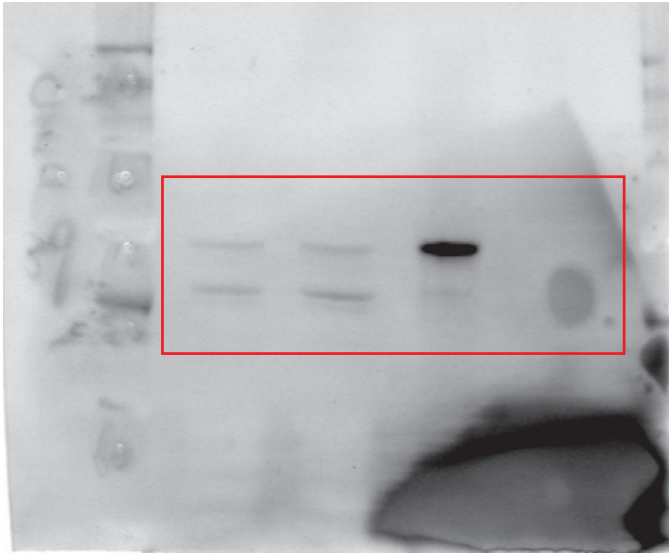
Figure 1-figure supplement1A_CEP89
