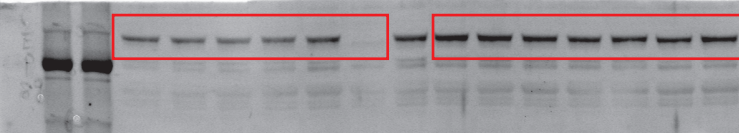
Figure 2-figure supplement 2A_CEP83
