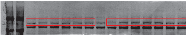
Figure 2-figure supplement 2A_ANKRD26
