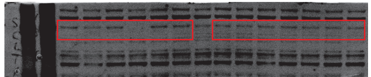
Figure 2-figure supplement 2A_IFT88
