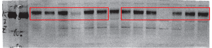
Figure 2-figure supplement 2A_NCS1
