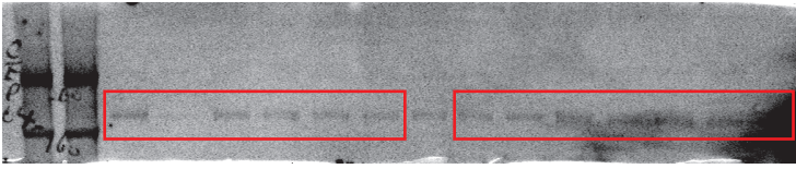
Figure 2-figure supplement 2A_CEP89
