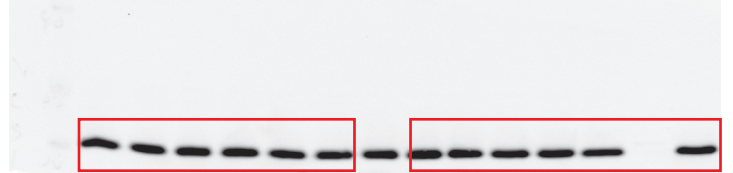
Figure 2-figure supplement 2A_SCLT1
