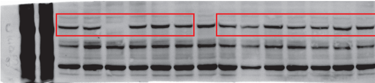
Figure 2-figure supplement 2A_CEP83
