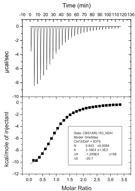
200 μM CNNM1 412-568 3 mM ARL15 32-197
