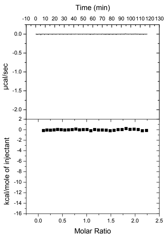
30 \mu\text{M} CNNM2 429-584 H523K 300 \mu\text{M} ARL15 32-197
