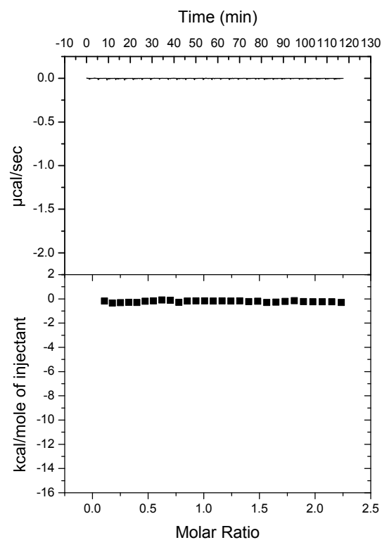
30 \mu\text{M} CNNM4 356-511 H450K 300 \mu\text{M} ARL15 32-197
