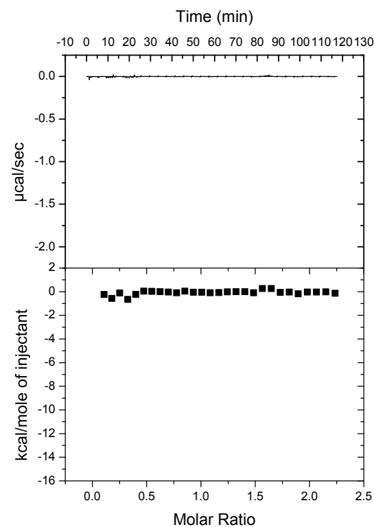
30 \mu\text{M} CNNM3 299-452 H391K 300 \mu\text{M} ARL15 32-197
