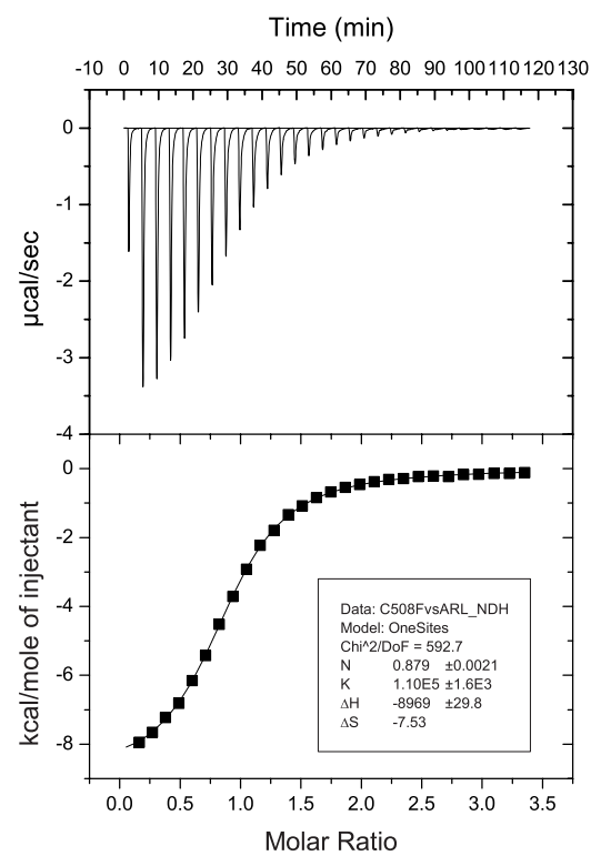
100 \mu\text{M} CNNM1 412-568 C508F 1.5 mM ARL15 32-197
