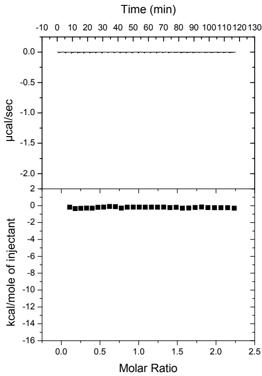
30 \mu\text{M} CNNM4 356-726 H450K 300 \mu\text{M} ARL15 32-197
