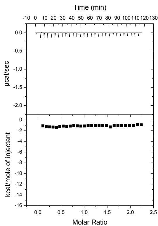
30 \mu\text{M} CNNM2 429-584 F524K 300 \mu\text{M} ARL15 32-197
