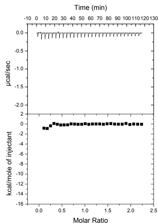
30 \mu\text{M} CNNM4 356-511 F451K 300 \mu\text{M} ARL15 32-197
