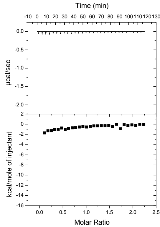
30 \mu\text{M} CNNM4 356-726 F451K 300 \mu\text{M} ARL15 32-197
