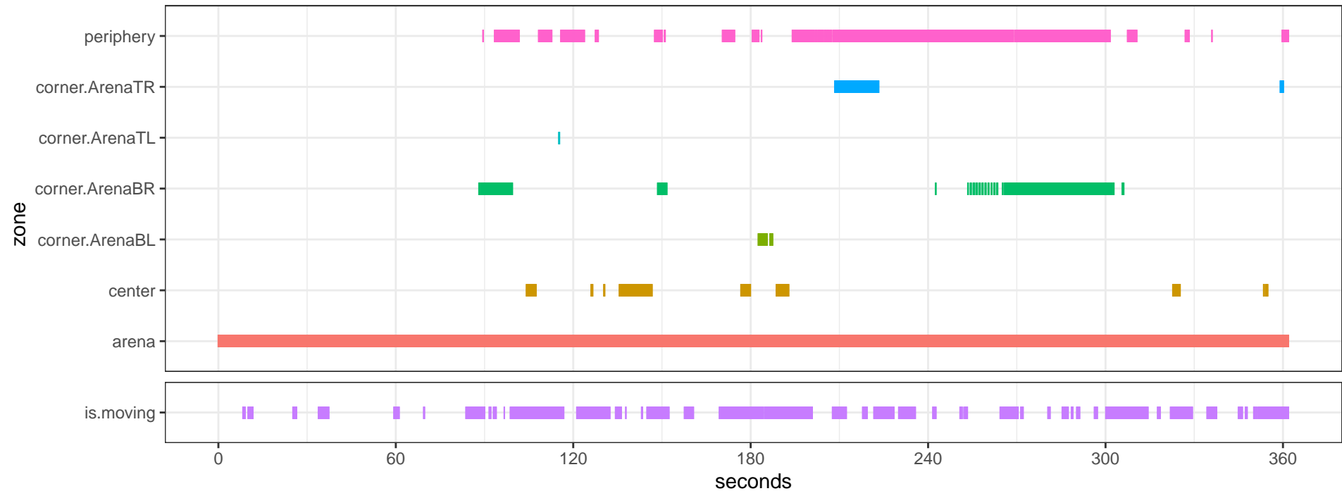
Maus_34-21_10_MAH00866DLC_resnet50_OpenFieldDec23shuffle1_600000_filtered.csv
