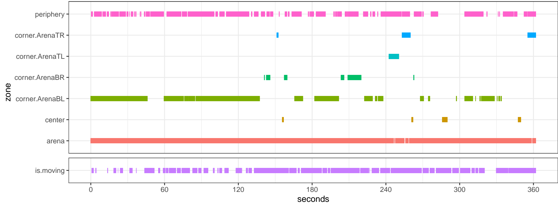
OF_top_Opto_52-LED1DLC_resnet50_OpenFieldDec23shuffle1_600000_filtered.csv
