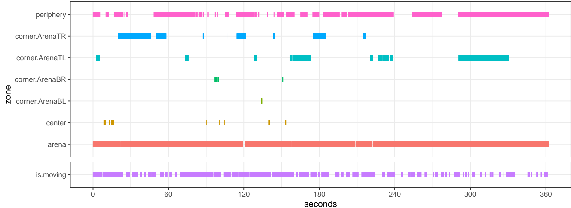
Maus_34-21_7_MAH00859DLC_resnet50_OpenFieldDec23shuffle1_600000_filtered.csv
