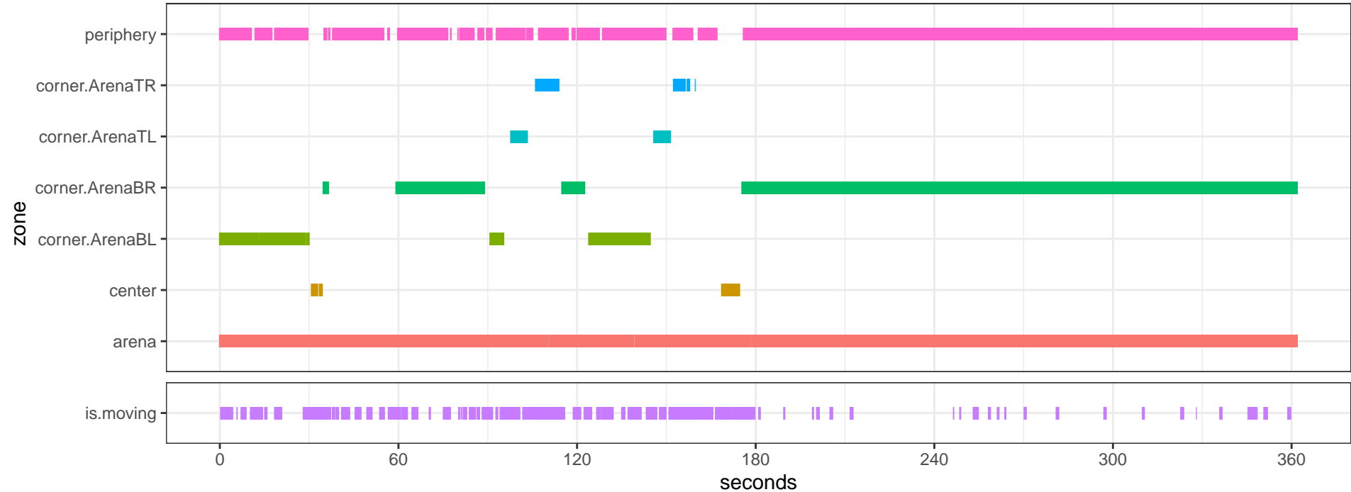
OF_top_Opto_61-LED1DLC_resnet50_OpenFieldDec23shuffle1_600000_filtered.csv
