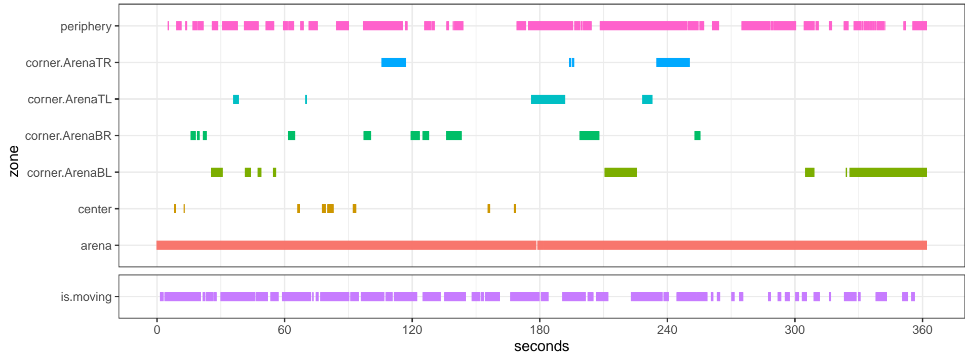
Maus_106-21_B_MAH01017DLC_resnet50_OpenFieldDec23shuffle1_600000_filtered.csv
