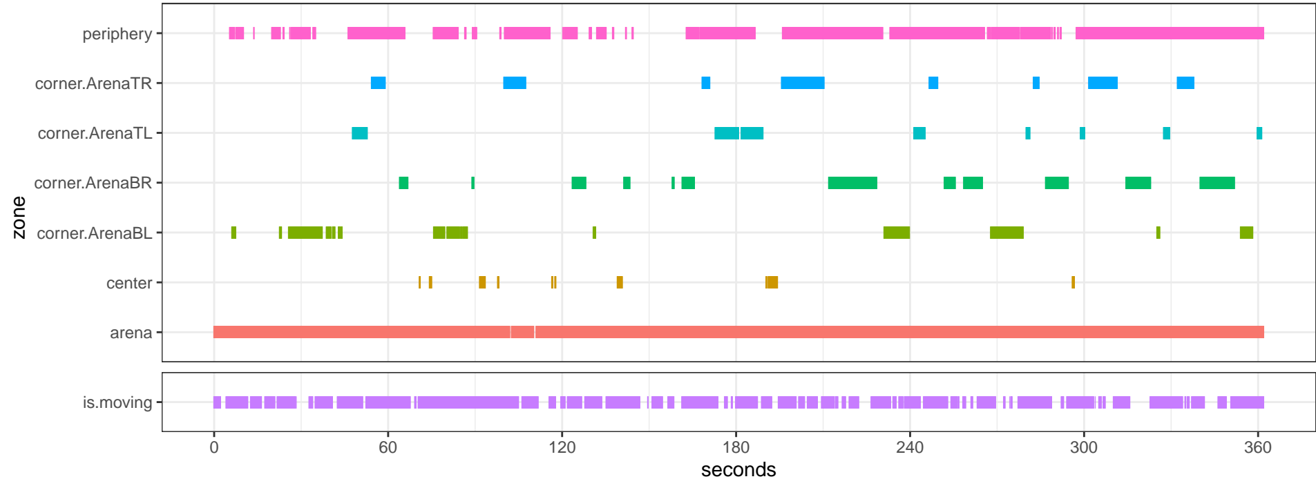
Maus_106-21_A_MAH01016DLC_resnet50_OpenFieldDec23shuffle1_600000_filtered.csv
