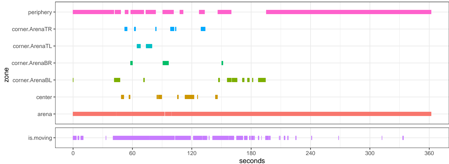
Maus_35E-20_LED1_MAH00338DLC_resnet50_OpenFieldDec23shuffle1_600000_filtered.csv
