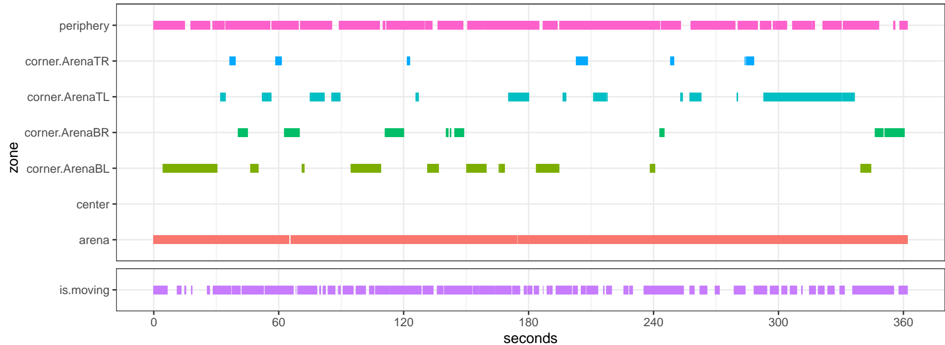
OF_top_Opto_75-LED1DLC_resnet50_OpenFieldDec23shuffle1_600000_filtered.csv
