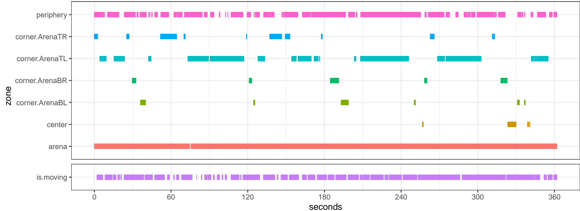
OF_top_Opto_15-LED1DLC_resnet50_OpenFieldDec23shuffle1_600000_filtered.csv
