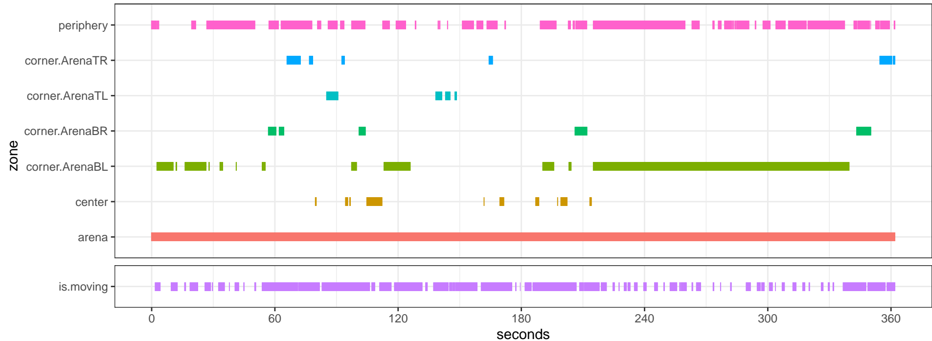
Maus_35A-20_LED1_MAH00335DLC_resnet50_OpenFieldDec23shuffle1_600000_filtered.csv
