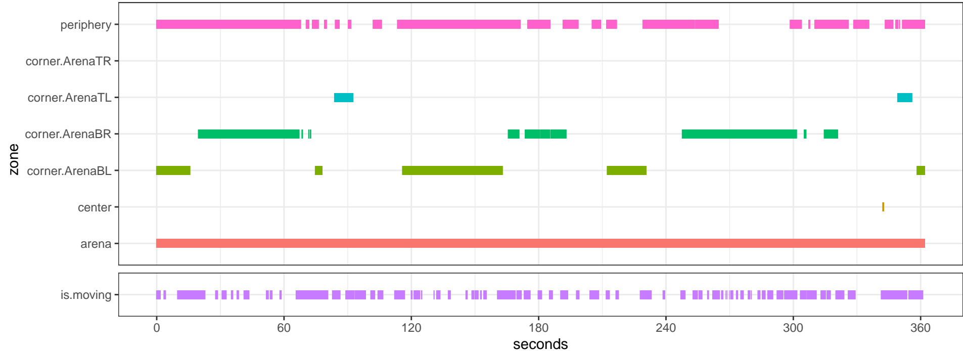
Maus_35C-20_LED1_MAH00336DLC_resnet50_OpenFieldDec23shuffle1_600000_filtered.csv
