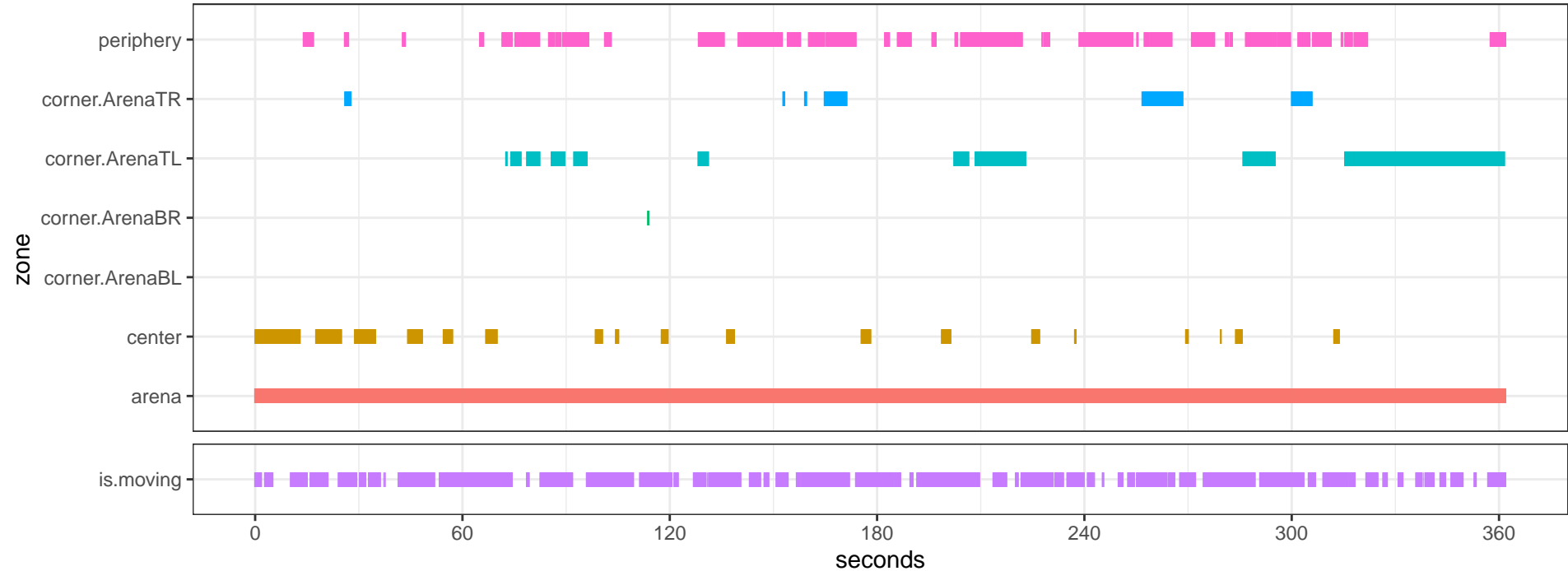
Maus_34-21_11_MAH00863DLC_resnet50_OpenFieldDec23shuffle1_600000_filtered.csv
