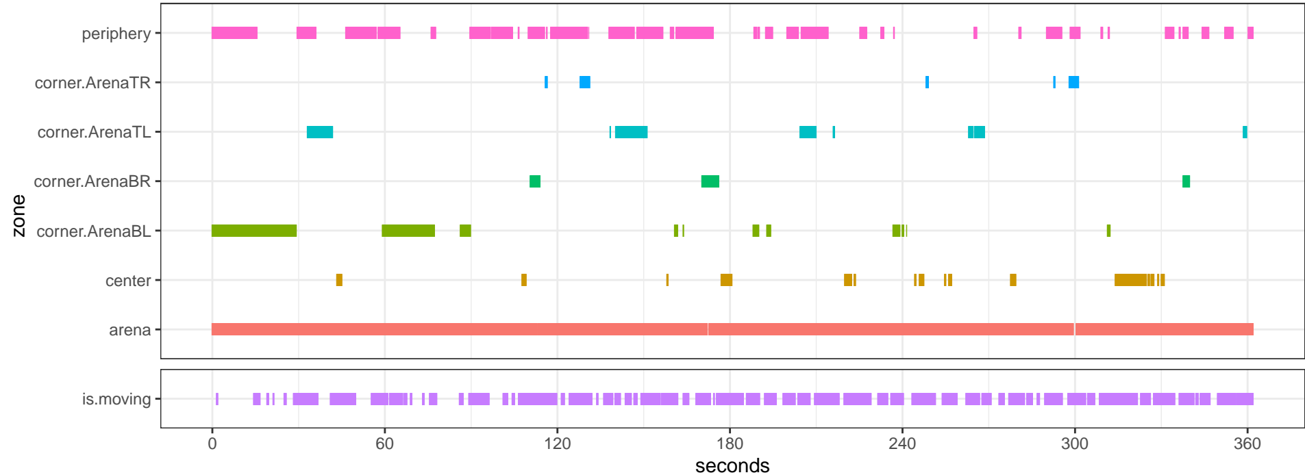
OF_top_Opto_10-LED1DLC_resnet50_OpenFieldDec23shuffle1_600000_filtered.csv
