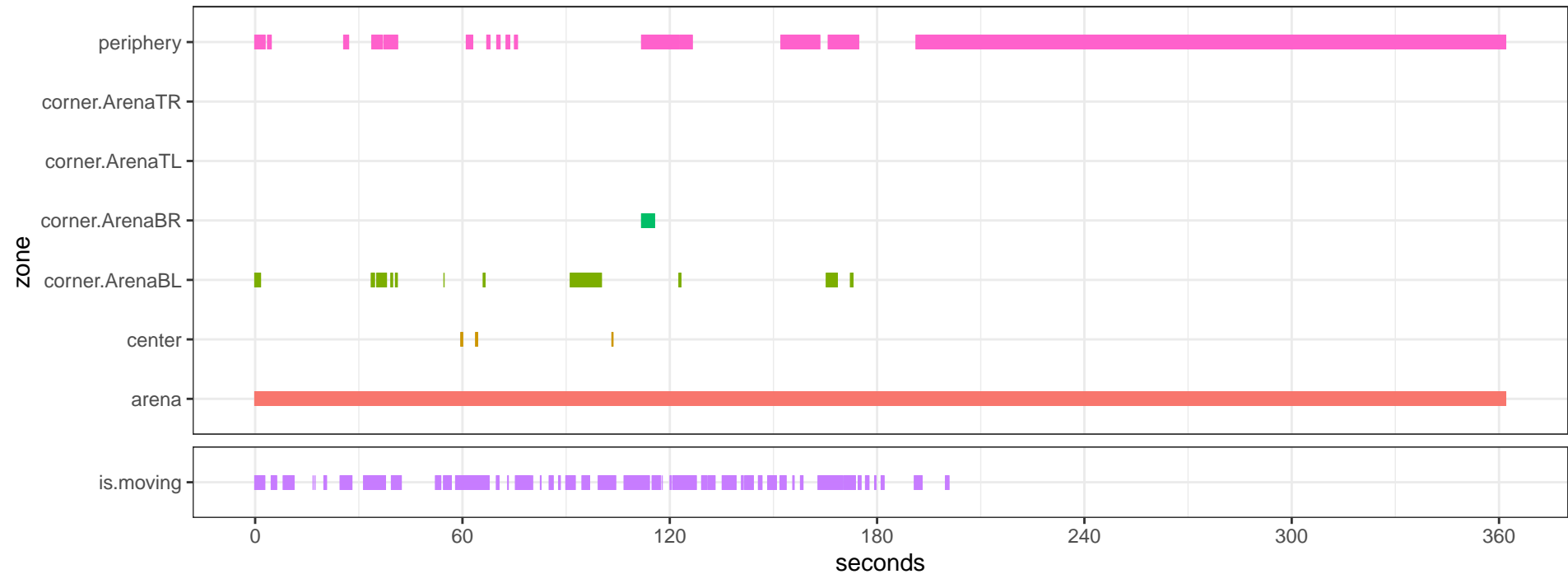
OF_top_Opto_76-LED1DLC_resnet50_OpenFieldDec23shuffle1_600000_filtered.csv
