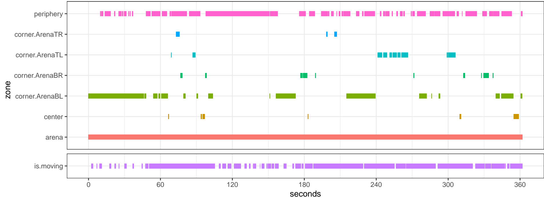
Maus_35D-20_LED1_MAH00337DLC_resnet50_OpenFieldDec23shuffle1_600000_filtered.csv
