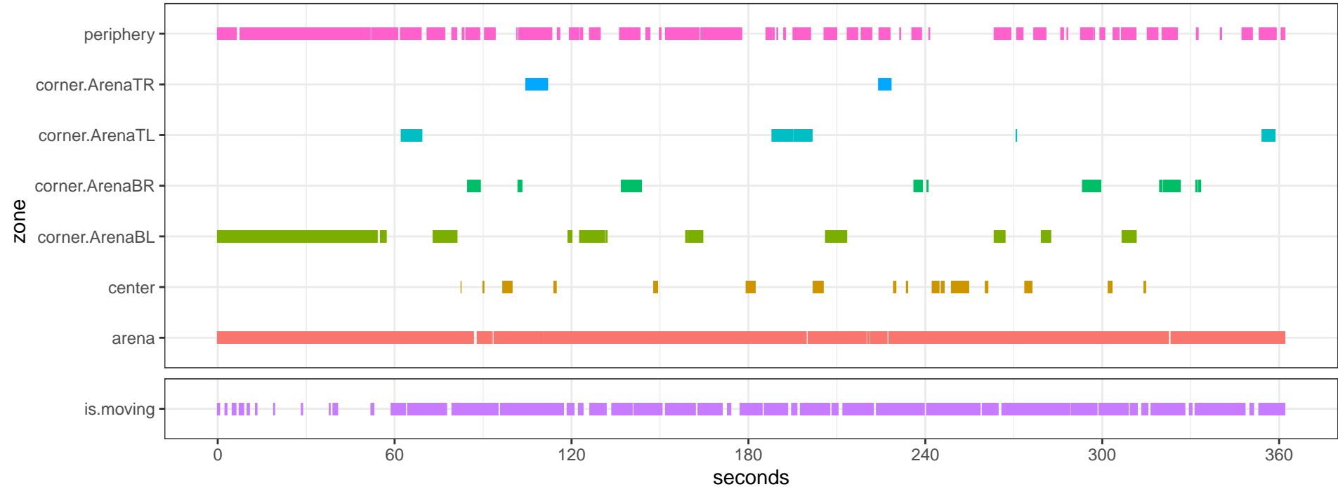
OF_top_Opto_11-LED1DLC_resnet50_OpenFieldDec23shuffle1_600000_filtered.csv
