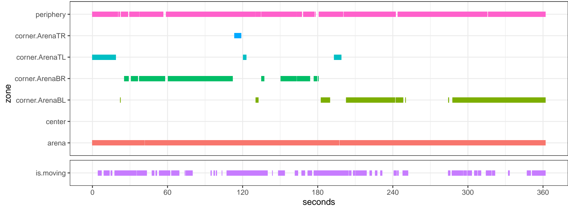
OF_top_Opto_04-LED1DLC_resnet50_OpenFieldDec23shuffle1_600000_filtered.csv
