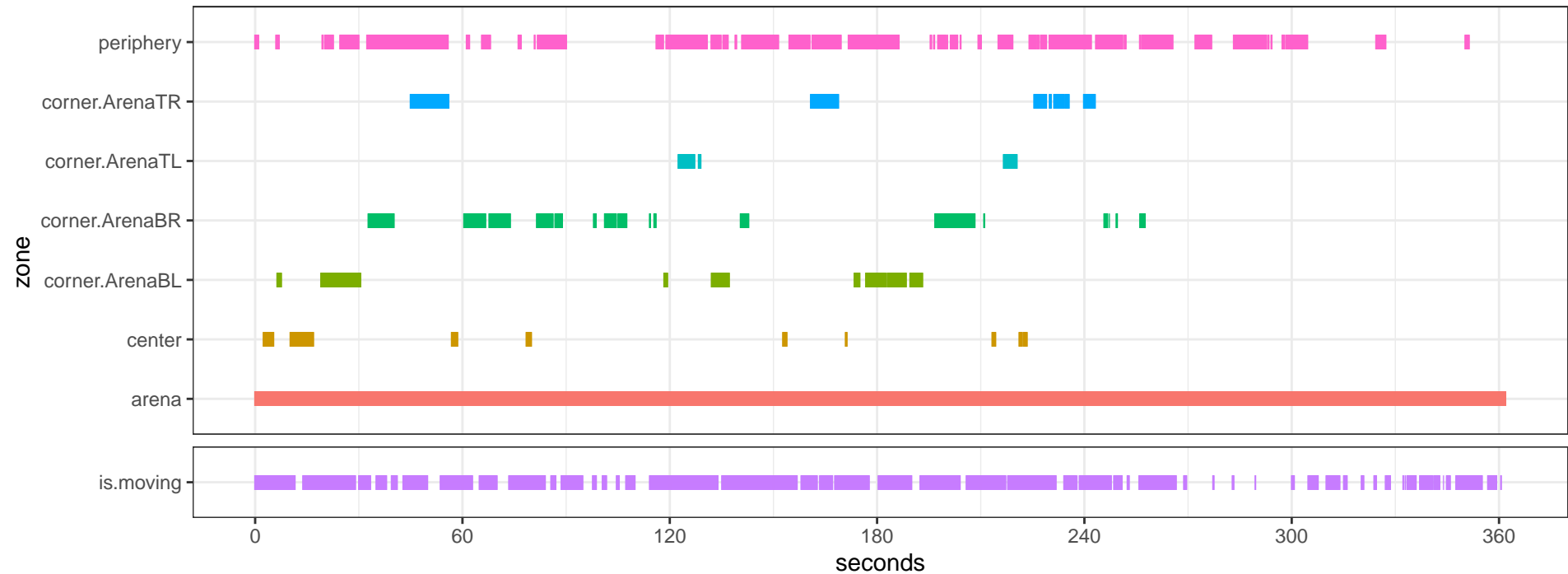
Maus_106-21_D_MAH01019DLC_resnet50_OpenFieldDec23shuffle1_600000_filtered.csv
