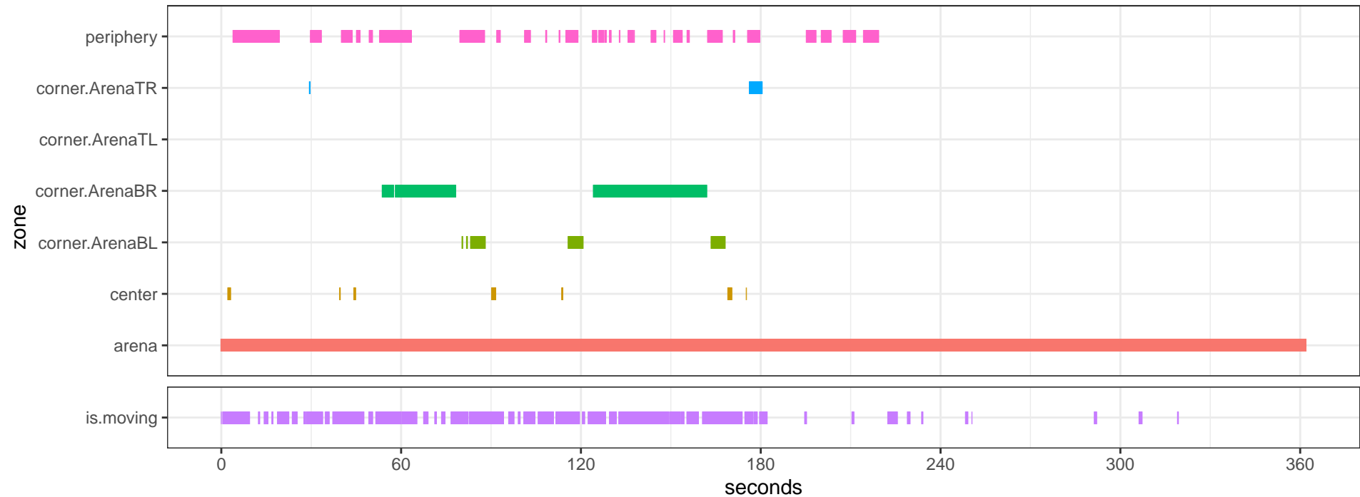
OF_top_Opto_77-LED1DLC_resnet50_OpenFieldDec23shuffle1_600000_filtered.csv
