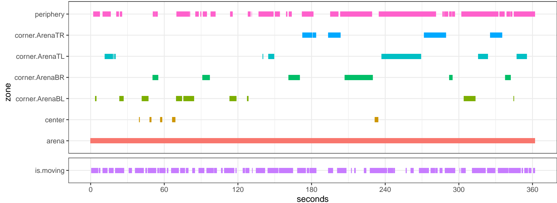
Maus_106-21_C_MAH01018DLC_resnet50_OpenFieldDec23shuffle1_600000_filtered.csv
