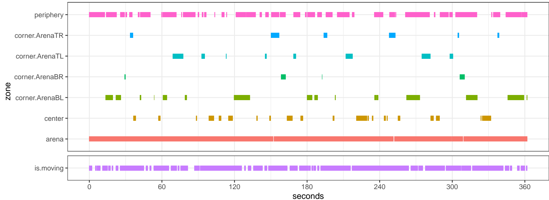
OF_top_Opto_16-LED1DLC_resnet50_OpenFieldDec23shuffle1_600000_filtered.csv
