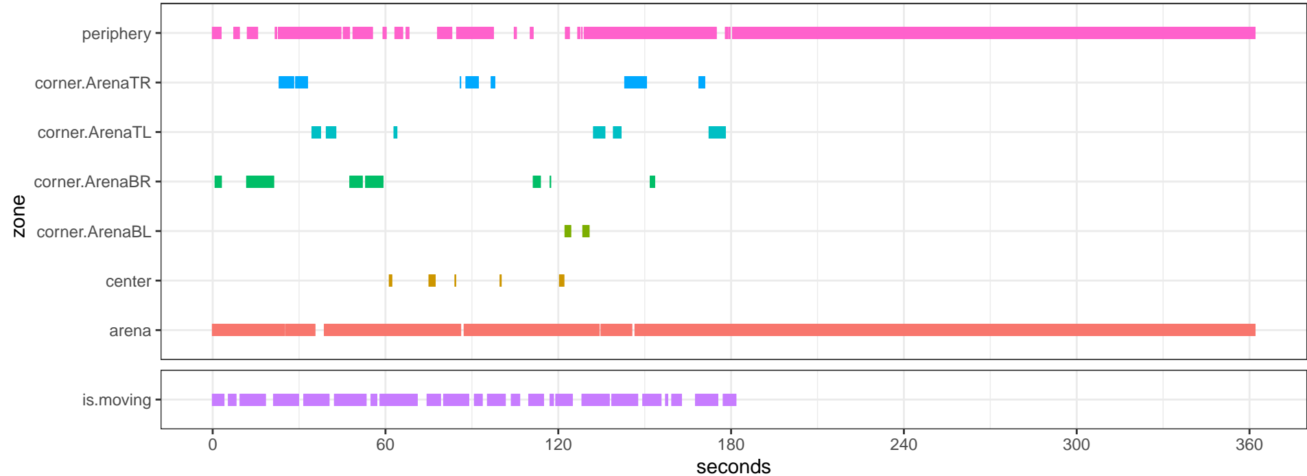
Maus_106-21_10_MAH01020DLC_resnet50_OpenFieldDec23shuffle1_600000_filtered.csv
