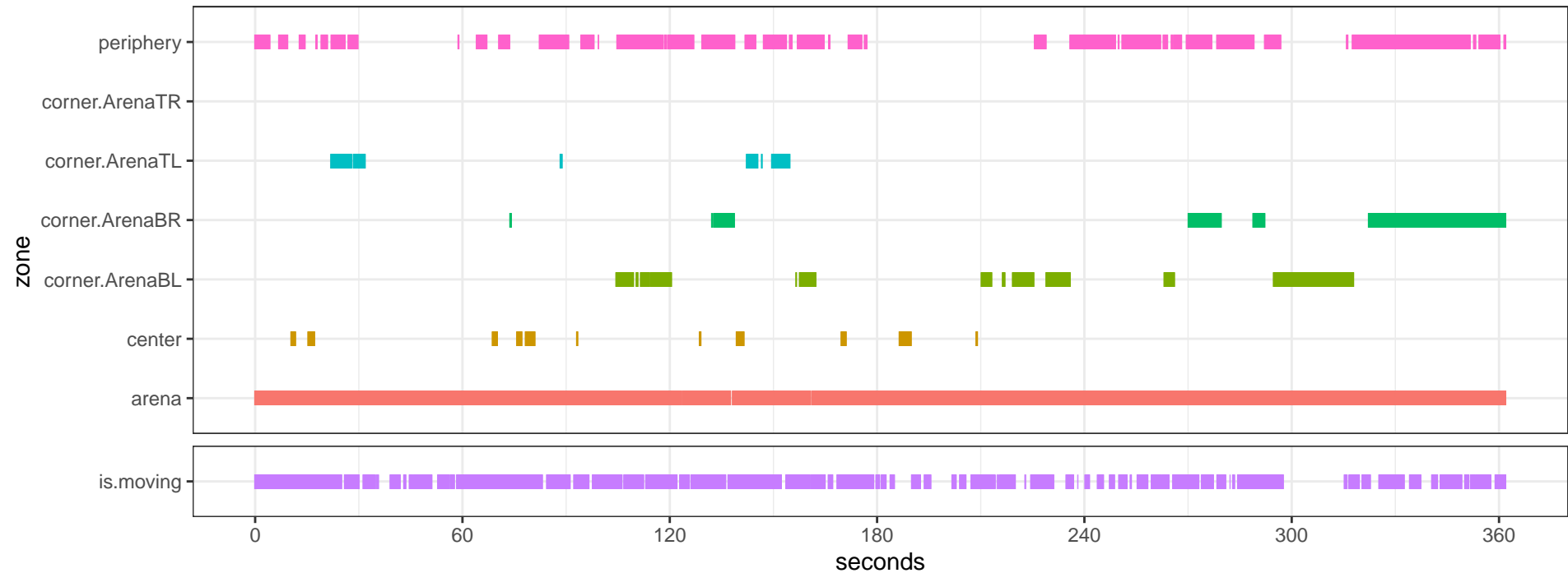
Maus_35B-20_LED1_MAH00339DLC_resnet50_OpenFieldDec23shuffle1_600000_filtered.csv
