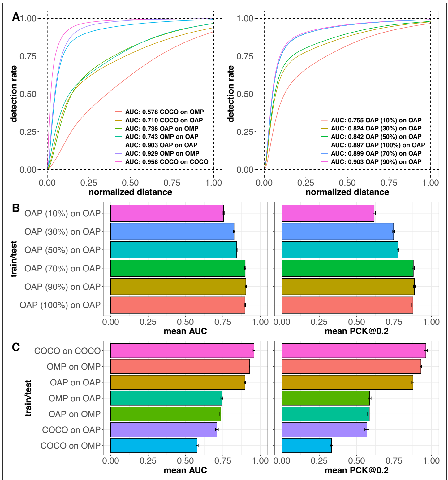
Figure 4. Keypoint detection performance of HRNet-W48 models on different datasets. (A) Keypoint detection performance of HRNet-W48 models measured using percent correct keypoints (PCK) values at different thresholds. Left: models trained on the full training sets of COCO, OpenApePose (OAP), and OpenMonkeyPose (OMP), and tested on the same dataset, as well as across datasets. Right: models trained on different sizes of the full OAP training set, and tested on the OAP testing set. (B) Barplots showing the keypoint detection performance of state-of-the-art (HRNet-W48) models as measured using percent keypoints correct at 0.2 (PCK@0.2) and area under the curve (AUC) of the PCK curves at thresholds ranging from 0.01 to 1. Error bars: standard deviation of the performance metrics. Models are trained on different sizes of the full training set of OAP and tested on held-out
