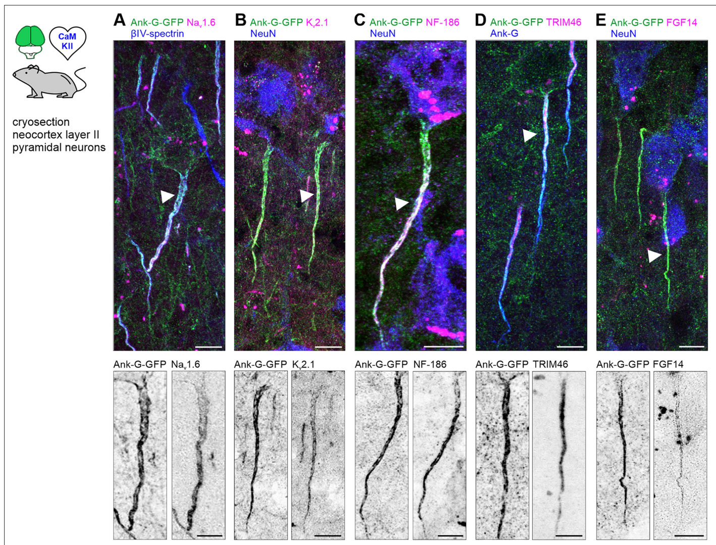
Figure 4. Ank-G-GFP expression does not affect the molecular axon initial segment (AIS) composition. (A) Merged image of layer II/III pyramidal neurons in S1 of an ank-G-GFP \times CaMKII-Cre mouse with intrinsic ank-G-GFP (green), co-labeled against \beta IV-spectrin (blue) and Nav1.6 (magenta). Bottom: Inverted black & white image of the ank-G-GFP (left) and Nav1.6 (right) signal in a single axon initial segment (AIS) (arrow in merged image). (B) Merged image of layer II/III pyramidal neurons in S1 of an ank-G-GFP \times CaMKII-Cre mouse with intrinsic ank-G-GFP (green), co-labeled against Kv2.1 (magenta) and NeuN (blue). Bottom: Inverted black & white image of the ank-G-GFP (left) and Kv2.1 (right) signal in a single AIS (arrow in merged image). (C) Merged image of a layer V pyramidal neuron in S1 of an ank-G-GFP \times CaMKII-Cre mouse with intrinsic ank-G-GFP (green), co-labeled against neurofascin-186 (magenta) and NeuN (blue). Bottom: Inverted black & white image of the ank-G-GFP (left) and NF-186 (right) signal in a single AIS (arrow in merged image). (D) Merged image of layer II/III pyramidal neurons in S1 of an ank-G-GFP \times CaMKII-Cre mouse with intrinsic ank-G-GFP (green), co-labeled against TRIM46 (magenta) and ankyrin-G (blue). Bottom: Inverted black & white image of the ank-G-GFP (left) and TRIM46 (right) signals in a single AIS (arrow in merged image). (E) Merged image of layer II/III pyramidal neurons in S1 of an ank-G-GFP \times CaMKII-Cre mouse with intrinsic ank-G-GFP (green), co-labeled against FGF14 (magenta) and NeuN (blue). Bottom: Inverted black & white image of the ank-G-GFP (left) and FGF14 (right) signal in a single AIS (arrow in merged image). All scale bars = 10 \mu m.
