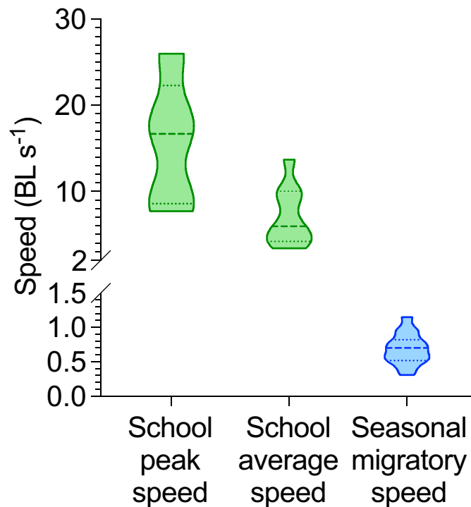
Appendix 1—figure 1. Swimming speeds of fish schools and seasonal migratory speeds in the open ocean. The figure is based on a summary of the swimming speed data from the literature (see Supplementary file 1 for details). We report the relative swimming speed (in body length per second, BL s -1 ) to account for the size range of species studied. We distinguished the data reported for peak speed and average speed for fish schools. Notably, schools can reach a peak speed that is nearly twice that of the average speed when they school actively in the ocean. Seasonal migratory speeds are most commonly obtained from animal-borne sensors, and data in the current literature currently skew toward large migratory species due to the technical limitations of attaching relatively large tags. Nevertheless, these are the best data available to estimate migratory speeds over long durations. A key criterion that we used in compiling these data is that the measurements are obtained from field settings e.g. estuaries and oceans. Our objective is to understand a wide range of swimming speeds of fish schools in natural habitats. This analysis demonstrates that fish schools often swim at high speeds (> 6 body length s -1 ) when moving in open-water habitats. According to the results of our metabolic testing, the high speeds of swimming observed in fish schools are sustained by a substantial amount of energy contributed by glycolytic metabolism. At higher speeds, our laboratory testing results demonstrate that schooling dynamics saved a substantial amount of total energy expenditure (TEE) when the energetic cost by fluid drag is at a premium. Data on seasonal migratory speeds also match our laboratory testing results showing that solitary individuals and fish schools have a minimum absolute energetic cost when swimming around ~1 BL s -1 . A version of this figure is published in Zhang and Lauder, 2023 .
