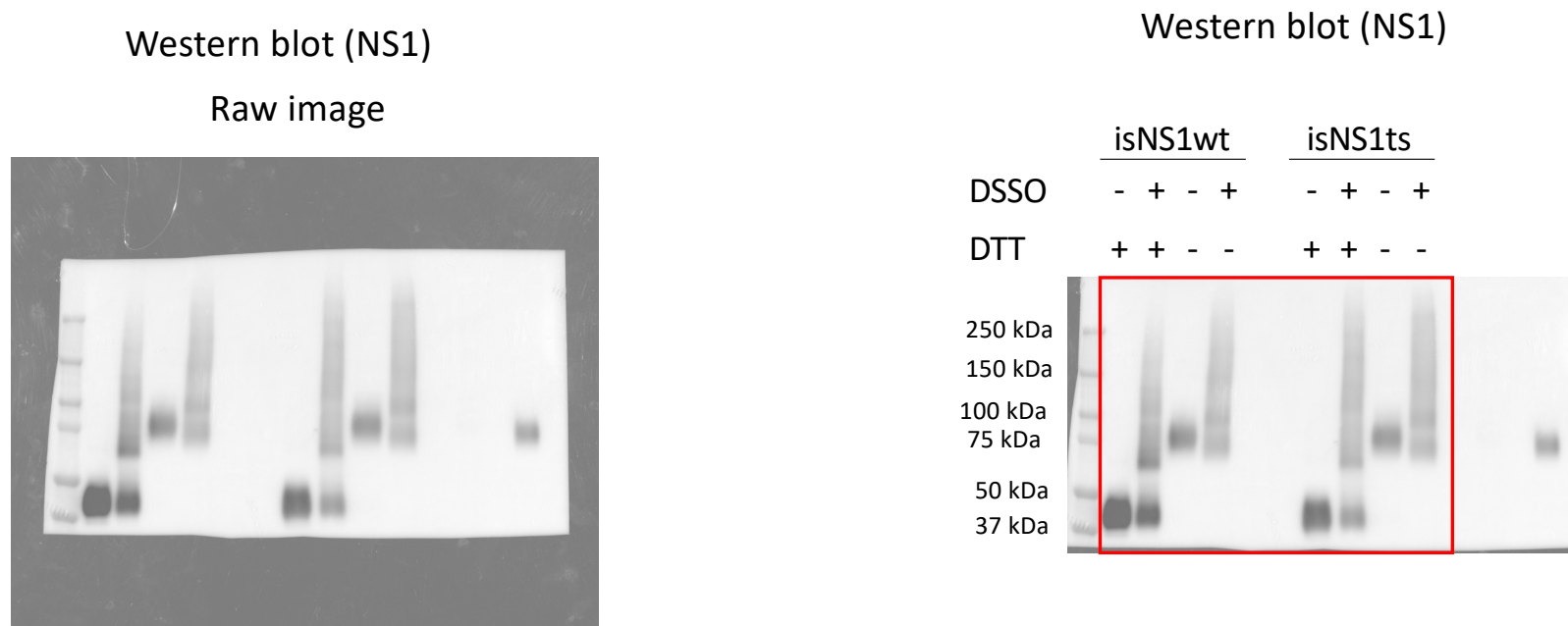
Figure 4-figure supplement 1-source data 1 Raw and annotated image for the western blot analysis (anti-NS1) on an SDS-PAGE gel
