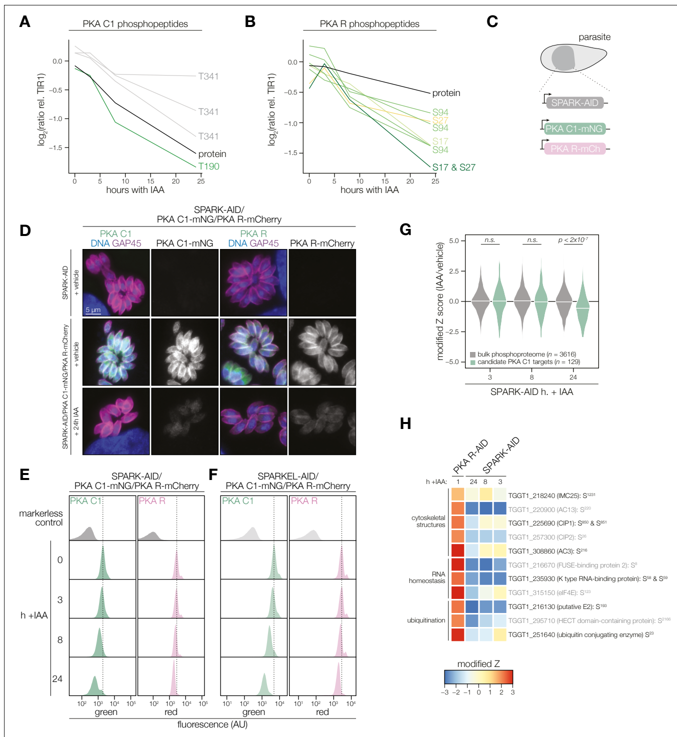
Figure 4. PKA C1 levels are down-regulated upon SPARK depletion. (A, B) Average protein and phosphopeptide abundances of PKA C1 (A) and PKA R (B) following SPARK depletion. (C) Schematic of the genetic strategy used to monitor PKA C1 and PKA R abundances following SPARK (or SPARKEL) down-regulation with IAA. (D) Immunofluorescence microscopy of parasites expressing SPARK-AID, PKA C1-mNG, and PKA R-mCherry after 0 or 24 hr of IAA treatment to degrade SPARK. Parasites and nuclei were stained with GAP45 and Hoechst 33342, respectively. GAP45 staining and mNG or mCherry staining were normalized to vehicle-treated tagged samples. (E, F) Flow cytometry analysis of parasites expressing PKA C1-mNG, PKA R-mCherry, and SPARK-AID or SPARKEL-AID, respectively, after the indicated period of IAA treatment. The dotted line centers the mode of the vehicle-treated sample. Traces were normalized by unit area. (G) Violin plots displaying the distribution of phosphopeptide abundance values following SPARK depletion. The distributions of candidate PKA C1 targets, as defined in the text and methods, are shown in green. The distributions and p-values (KS
