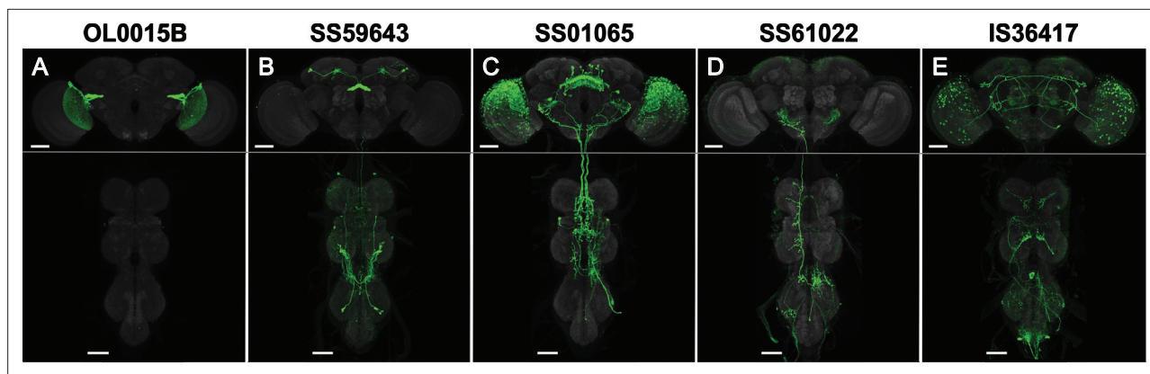
Figure 2. Examples of line quality levels. The 3060 cell-type lines were scored for expression. (A) Quality level 1 (1767 lines): Split-GAL4 line OL0015B (Wu et al., 2016) is specifically and strongly expressed in a single cell type. Occasional weak expression may be seen in other cells. (B) Quality level 2 (1232 lines): Split-GAL4 line SS59643 (Wolff et al., 2024) has expression in two cell types. Occasional weak expression may be seen in other cells. (C) Quality level 3 (26 lines): Split-GAL4 line SS59643 (Wolff et al., 2024) has expression in three or more cell types. (D) Quality level 4 (34 lines): Split-GAL4 line SS61022 has specific expression but weak or variable labeling efficiency. See Figure 2—figure supplement 1 for examples of variable expression. (E) Quality level 5: IS36417 is an Initial Split combination not selected for stabilization. Groups of neurons are visible, but the cell type of interest was not labeled with sufficient specificity for further work. Such lines were only included in the raw image collection. Scale bars, 50 \mu m.
